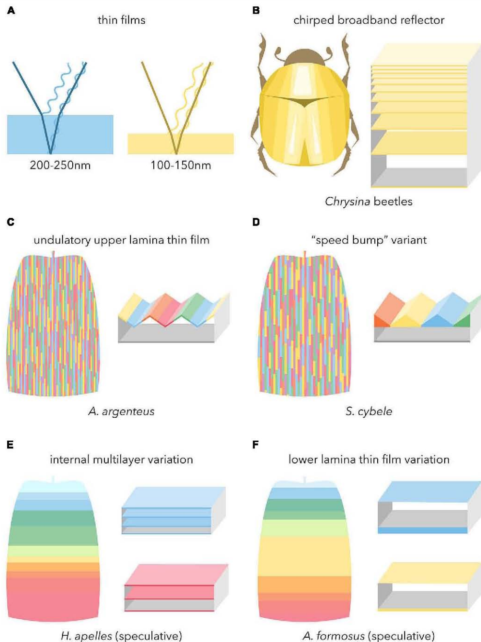
FIGURE 7 | Broadband reflectors underlying metallic iridescence in butterflies. Boxed schematics feature high-refractive index (filled) and low-refractive index (empty) materials. (A) Basic configuration of light reflection in simple chitinous thin-films. (B) Thick chirped stack reflector as observed in metallic beetles and butterfly pupae (after Neville, 1977). (C,D) Undulatory thin-films coupling a sawtoothed upper surface with an inner air layer, including the newly described variant from fritillary butterflies. Color array depicts the resulting rod-like mode of additive color mixing as observed under epi-illumination ( Figures 4G–H ; see also Vukusic et al., 2008). (E,F) Speculative modes of proximo-distal additive color mixing as observed in a silvery lycaenid and golden riodinid (see main text for details).
