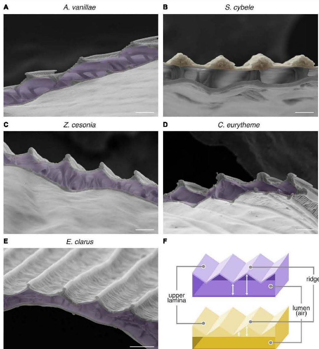
FIGURE 5 | Internal scale anatomy of nymphalid, pierid, and hesperid undulatory thin-film reflectors. (A–E) SEM of transverse sections of the metallic scales of A. vanillae , S. cybele , Z. cesonia , C. eurytheme , and E. clarus reveal the undulatory profile of the specular thin-film. False colors highlight the layer with the most consistent fluctuation in thickness, i.e., the air lumen (purple) in most cases, or for S. cybele , the thickened ridge regions (yellow). (F) Schematic representation of the two types of thin-film thickness undulation as observed in panels (A,C–E) (top, purple) and (B) (bottom, yellow). Scale bars: (A–E) = 1 \mu m.
