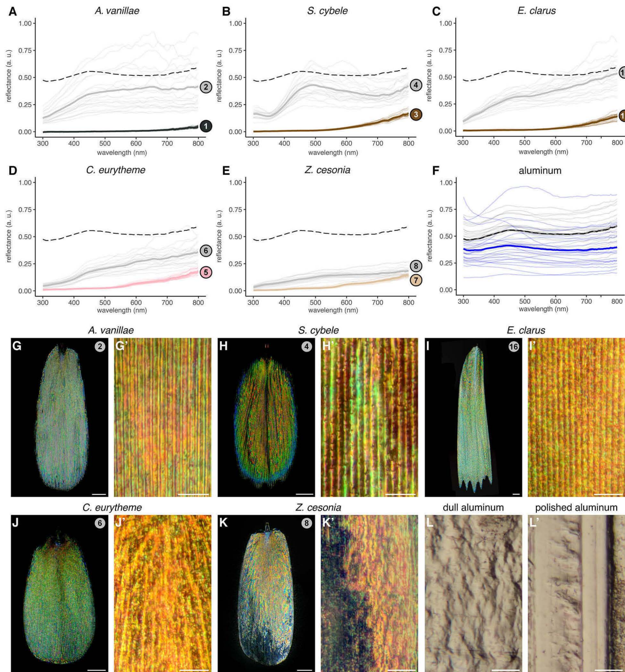
FIGURE 4 | Silver broadband reflectance resulting from densely intermixed colored reflections. (A–E) Reflectance spectra of silver pattern elements (gray lines), compared to adjacent arrays of non-reflective scales (black, brown, pink and beige lines). Faded lines represent individual measurements taken within the same wing surface. Dotted lines indicate the averaged spectra of polished aluminum foil for comparison. (F) Reflectance spectra of the polished side (gray) and dull side (blue) of aluminum foil. (G–K') High-magnification reflected-light microscopy of single silver scales using a MPlanFLN 50 lens (G–K) , and an LMPlan Achromatic 100 lens (G'–K') . (L, L') High magnification reflected light microscopy of dull and polished sides of aluminum foil under the 100 lens. Scale bars: (G–K) = 20 \mu m; (G'–K', L, L') = 10 \mu m.
