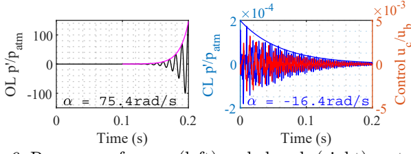
Fig. 6. Response of open- (left) and closed- (right) systems at b=0.3m and x_0=0.041m to a unit impulse input
