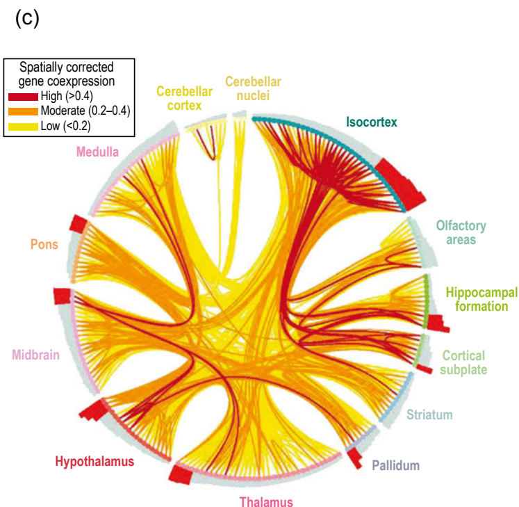
Figure 9.3 (continued) (c) Brain regions have been arranged around a circle, ordered by number of connections (bars) in each anatomical subdivision. Hubs are marked by red bars. The connection diagram traces anatomical connections between pairs of brain regions, color-coded by the corresponding gene co-expression value, after applying a correction for spatial distance. Statistical analysis revealed strongest gene co-expression among pairs of regions linked by reciprocal connections (as compared with unidirectional or unconnected pairs), as well as for rich connections linking hubs (as compared with feeder and peripheral connections). Genes driving correlations in expression in connections involving hub regions are functionally enriched in oxidative energy metabolism. Connectivity data derived from Bassett and Sporns (2017).
