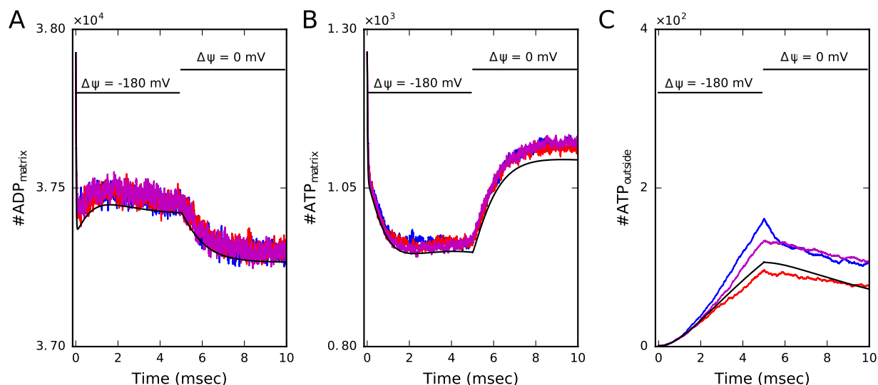
Figure 6. Dependence on the mitochondrial membrane potential. In this configuration we start our simulations with a functional mitochondrion in the same scenario as in Fig. 4 and at 5 milliseconds we emulate the breakdown of the membrane potential from \Delta\psi = -180 mV to \Delta\psi = 0 mV by changing the corresponding protein activity rates (Supplementary Tables 2 and 3). Under these conditions ATP synthases work stochastically in a reversible form hydrolyzing and phosphorylating ATP, leading on average to a reduction in the number of ADP in the matrix (A) and to an increase in the number of ATP in the matrix (B). Overall, under these conditions the capacity of the organelle to produce ATP is abolished and no more ATP molecules reach the outside (C).
