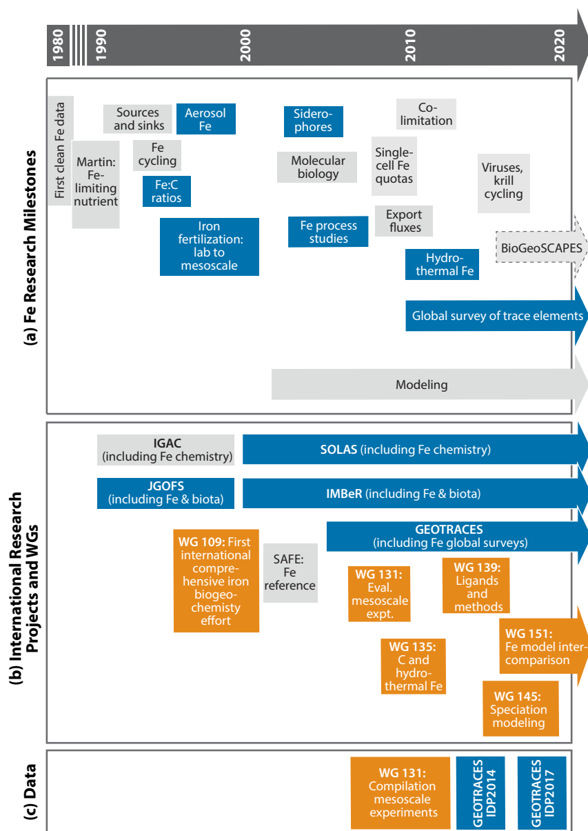
FIGURE 1. Timeline of SCOR contributions to advancing understanding of iron chemistry in seawater. Activities sponsored by SCOR are in blue. SCOR-sponsored working groups are in orange. Projects not supported directly by SCOR are gray. (a) Milestones reached in relevant global research projects and topics. BioGeoSCAPES ( https://www.biogeoscap.es.org/ ) is represented with a dashed arrow, as it is a developing project that could contribute new understanding of the role of organisms in the global iron cycle. (b) Major developments in advancing understanding of iron chemistry in the ocean, including contributions from SCOR-sponsored research projects and SCOR Working Groups. (c) SCOR-sponsored contributions to data.
