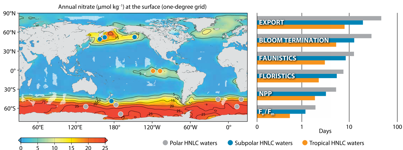
FIGURE 2. Locations of in situ mesoscale iron enrichment studies in polar (gray symbols), subpolar (blue symbols), and tropical (orange symbols) high nitrate-low chlorophyll waters, along with a summary of the timescales of biological responses. The left panel overlays the location of each study on a map of global ocean surface nitrate concentrations. Nitrate concentrations courtesy of NOAA's National Oceanographic Data Center. The right panel summarizes timescales of biological responses (log time scale, 0 denotes iron release), from photosynthetic to biogeochemical, following purposeful mesoscale iron enrichment. F_v/F_m is phytoplankton photosynthetic competence, and NPP denotes net primary production. Bloom termination is defined as the period during which a sustained decrease in bloom stocks is observed. Export is defined as enhancement of the downward flux of particles in the upper 300 m. The temporal trends demonstrate that different locales have characteristic response times. Data are available from the BCO-DMO relational database ( https://www.bco-dmo.org/program/2017 ). Figure modified from Boyd et al. (2012)
