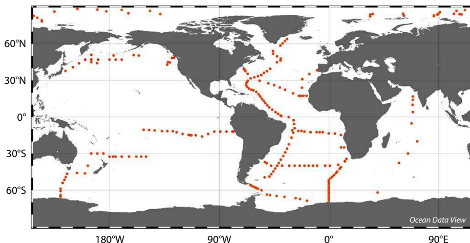
FIGURE 3. Locations of GEOTRACES stations with iron data, from the surface to the seafloor (IDP-2017; Schlitzer et al., 2018), including data through 2016. Figure courtesy of Reiner Schlitzer (AWI)
