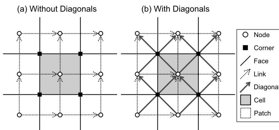
Figure 1. Grid elements of RasterModelGrid without (a) and with (b) diagonals.
