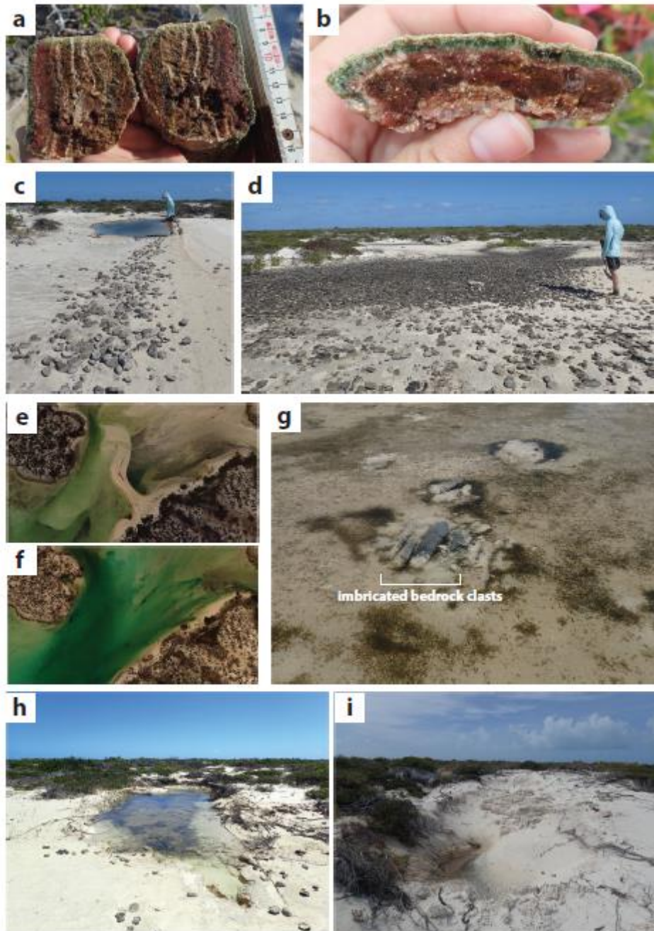
Figure 6: Images of erosional sedimentary features of Hurricane Irma on LAC. (A, B) Cross-sections of microbial mat intraclasts illustrating rounded edges due to erosion and varying morphologies—equant (A) and tabular (B). (C, D) Lag deposits of microbial mat intraclasts, which can range from relatively small spatial extent and intraclast density (C) to larger spatial extent with high density of intraclasts (D). (E, F) Drone images illustrating extensive scour in tidal channels: (E) channel imaged prior to Hurricane Irma and (F) after Hurricane Irma, when the entire channel was scoured to >3 m water depth. (G) Examples of lithified clasts transported into island interior, illustrating rare example of imbricated clasts. (H, I) Scour pits near washover fans, including representative morphologies of scour pits located immediately adjacent to washover fan and >1 m deep scour in the lithified beach ridge to the south of washover fans.
