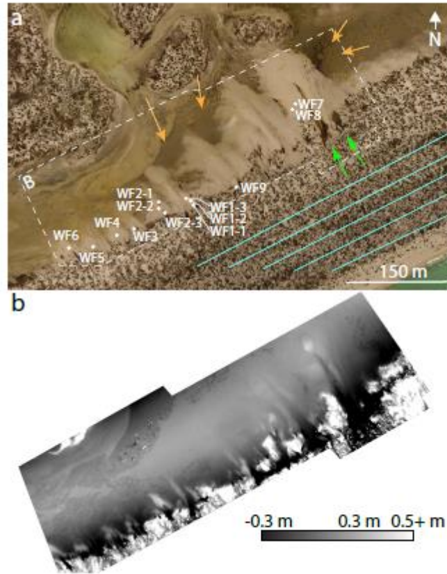
Figure 3: (a) Washover fan sample locations and (b) digital elevation model of the washover fan area. In (a), turquoise lines indicate the beach ridge area and green arrows indicate two of the larger scour pits. Scour pits are present adjacent to each of the washover fans on either side. Major microbial mat areas adjacent to the washover fans are indicated by orange arrows.
