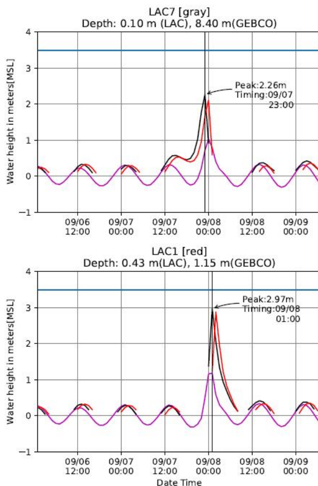
Figure 2: Time series of simulated storm surges in meters above mean sea level around Little Ambergris Cay during Hurricane Irma (September 2017). Representative stations at the north and south side of the island are shown here.
