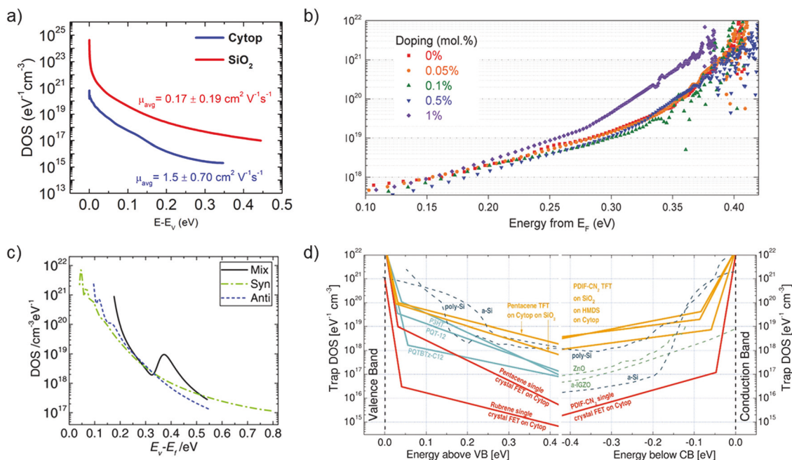
Fig. 10 (a) Comparison of the interfacial trap DOS spectrum for diF-TES ADT films with Cytop (blue) and SiO 2 (red) dielectrics evaluated using Gr unewald's model. The value of mobility is listed in the inset. Adapted with permission from ref. 97, Copyright 2015, AIP Publishing LLC. (b) Effect of p-doping on the trap DOS of OSC/polymer blend OFETs evaluated using Gr unewald's model. Reproduced with permission from ref. 198, Copyright 2017, Wiley-VCH. (c) Effect of isomer purity of diF-TES ADT on the trap DOS spectrum determined using Method II by Kalb et al. Broken green and blue curves represent trap DOS of pure syn - and anti -isomers respectively while the solid black lines represent that of the mix sample for reference. Reproduced with permission from ref. 205, Copyright 2017, Wiley-VCH. (d) Comparison of the interfacial trap DOS for several organic and inorganic FETs calculated using the numerical method by Oberhoff et al. Reproduced with permission from ref. 208, Copyright 2010, American Physical Society.
