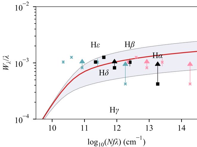
Figure 2. Curve-of-growth analysis of the Balmer absorption lines. Only H\beta , H\delta , and H\epsilon are used in the fit. The best-fit curve with b = 313 \text{ km s}^{-1} , C = 0.25 , and \log_{10}N = 17.6 \text{ cm}^{-2} is shown in red. The shaded area shows the region bounded by the 1\sigma uncertainty in the Gaussian parameter ( \sigma_b = 170 \text{ km s}^{-1} ). We also plot our data with \log_{10}N = 16.6 \text{ cm}^{-2} (green) and \log_{10}N = 18.6 \text{ cm}^{-2} (pink) on the growth curve. In this high-opacity regime ( \tau > 1 ), the EW is insensitive to N .
