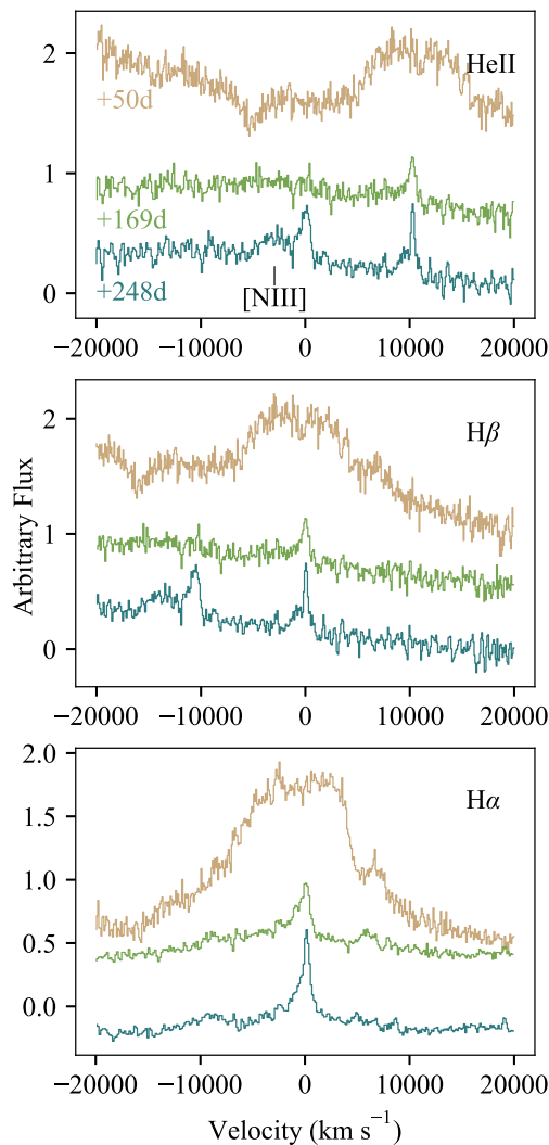
Figure 8. Velocity profiles of He II \lambda 4686 , H\beta , and H\alpha of AT2018zr at \Delta t = 50, 169 , and 248 days. Narrow H\alpha , H\beta , and He II \lambda 4686 emission emerged 6 months after maximum light. The narrow line widths are on the order of 1000 \text{ km s}^{-1} , which is only \sim 10\% of the broad Balmer line widths from earlier epochs. We note that on day 50, H\alpha and H\beta have a similar velocity profile that is dented on the red wing, which is likely to arise from the geometry of the line-forming region.
