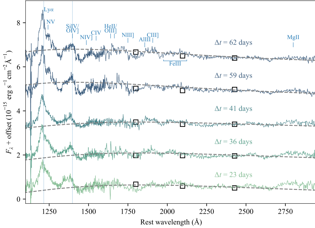
Figure 3. The HST STIS spectra of AT2018zr observed at different epochs, where \Delta t indicates the rest-frame time elapsed since the peak in the r band (MJD 58,194.5). To guide the eye, the gray dashed line marks the tentative FUV continuum extrapolated from a blackbody spectrum that is used to describe the NUV and optical SED. The blackbody spectra correspond to a temperature of T = 1.7 \times 10^4 K for the first three epochs and T = 2.2 \times 10^4 K for the last two epochs. The black squares indicate the interpolated broadband flux measured by Swift .
