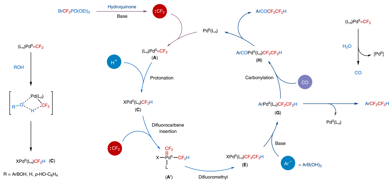
Fig. 5 | Outline of a possible pathway for controllable palladium-catalysed difluorocarbene transfer. The reaction is initiated by the formation of palladium(0) difluorocarbene complex A , in which the difluorocarbene is generated by the reaction of \text{BrCF}_2\text{PO}(\text{OEt})_2 with hydroquinone in the presence of base. Subsequent protonation at the difluorocarbene carbon of A gives the key intermediate C , which is illustrated in more detail at the lower left of the figure. As a process competitive to \text{CF}_2 elongation, C undergoes transmetalation and reductive elimination to produce \text{ArCF}_2\text{H} , depending on the tuning of the reaction conditions (Supplementary Figs. 8, 11 and 12). Difluorocarbene insertion into C forms palladium difluorocarbene complex A' , and then intermolecular difluoromethyl migration generates \text{CF}_2 elongated complex E . Subsequent transmetalation of E produces complex G , which undergoes reductive elimination to provide tetrafluoroethylated arenes. Alternatively, insertion of CO, which originates from the hydrolysis of [\text{Pd}^{\text{II}}]=\text{CF}_2 (as shown in the upper right of the figure), into the \text{Pd-Ar} \sigma bond of G , followed by reductive elimination, gives tetrafluoroethyl aryl ketones. In another competitive reaction, the key intermediate C may also undergo carbonylation to afford difluoromethyl aryl ketones (Supplementary Figs. 8 and 13). For simplicity, all palladium complexes are illustrated as neutral species, and all processes are depicted as being irreversible. \text{L}_n denotes Xantphos coordinated to palladium.
