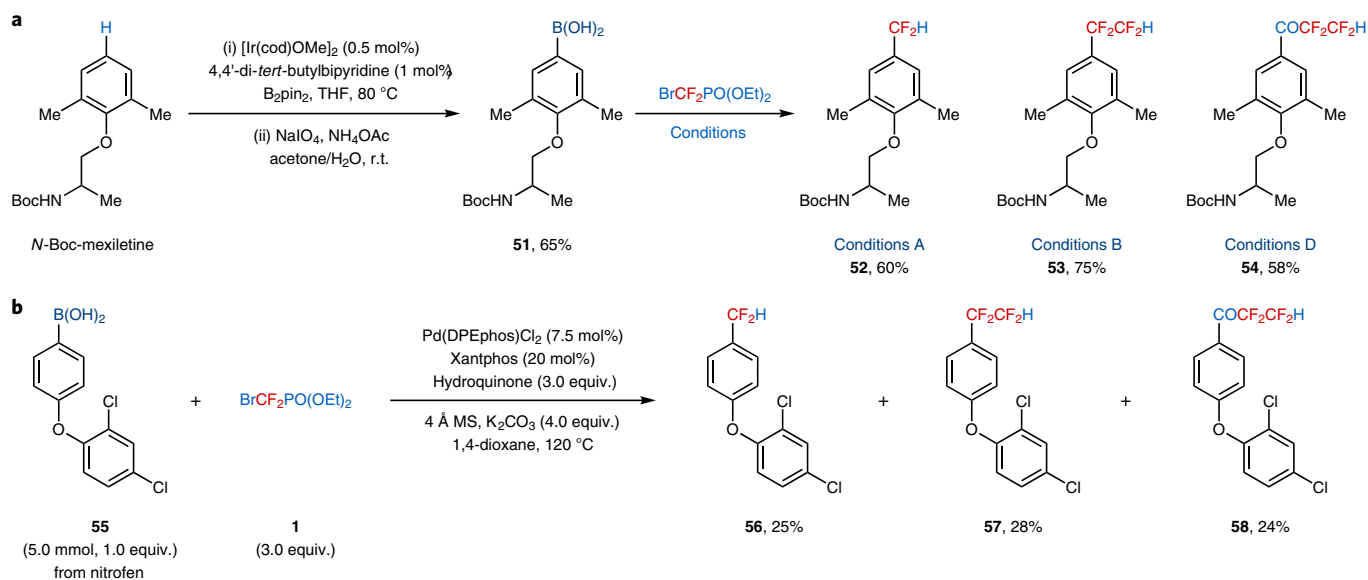
Fig. 2 | Diversified synthesis of fluoroalkylated arenes. a , Selective C–H bond borylation and fluoroalkylation of pharmaceuticals. Mexiletine, an anti-arrhythmic drug, can be readily modified to selectively provide three mexiletine analogues through the presented late-stage strategy. b , One-pot diversity-oriented modification of agrochemicals. Nitrofen, a herbicide, can be readily modified from one simple starting material to provide three diversified fluoroalkylated nitrofen analogues. Isolated yields are shown. B 2 pin 2 , 4,4,4',4',5,5,5',5'-octamethyl-2,2'-bi(1,3,2-dioxaborolane). DPEphos, (oxybis(2,1-phenylene))bis(diphenylphosphane).
