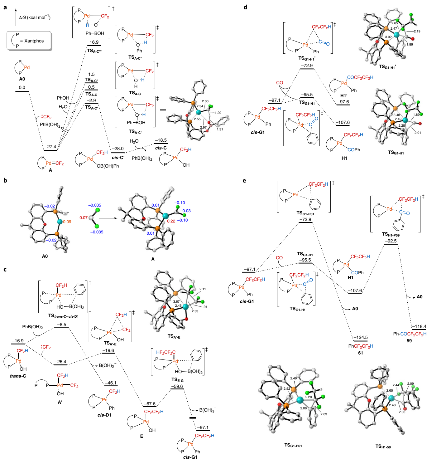
Fig. 4 | Calculated energy profile of the palladium-catalysed difluorocarbene transfer reactions. a , DFT-computed reaction pathways and optimized key transition state structures for protonation of [(\text{Xantphos})\text{Pd}^0=\text{CF}_2] A . Here, we chose cis - [(\text{Xantphos})\text{Pd}^0(\text{CF}_2\text{H})(\text{OH})] ( cis-C ) as the protonation intermediate in calculations (also in c ), because its transmetalation has a lower barrier than the direct transmetalation of [(\text{HCF}_2)(\text{Xantphos})\text{Pd}^0[\text{PhB}(\text{OH})\text{O}]] ( cis-C' ) (Supplementary Figs. 11 and 12). b , Computed charge model 5 (CM-5) charges of (\text{Xantphos})\text{Pd} , difluorocarbene and [(\text{Xantphos})\text{Pd}^0=\text{CF}_2] A . c , Free energy barrier differences between difluorocarbene insertion and transmetalation of trans-C . d , DFT-computed reaction pathways and optimized key transition state structures for insertion of CO into complex G1 . e , Free energy barrier differences between reductive elimination and CO insertion of complex G1 . Colour code: grey, carbon; white, hydrogen; blue, palladium; orange, phosphorus; red, oxygen; green, fluorine; pink, boron. All energies are reference to A0 .
