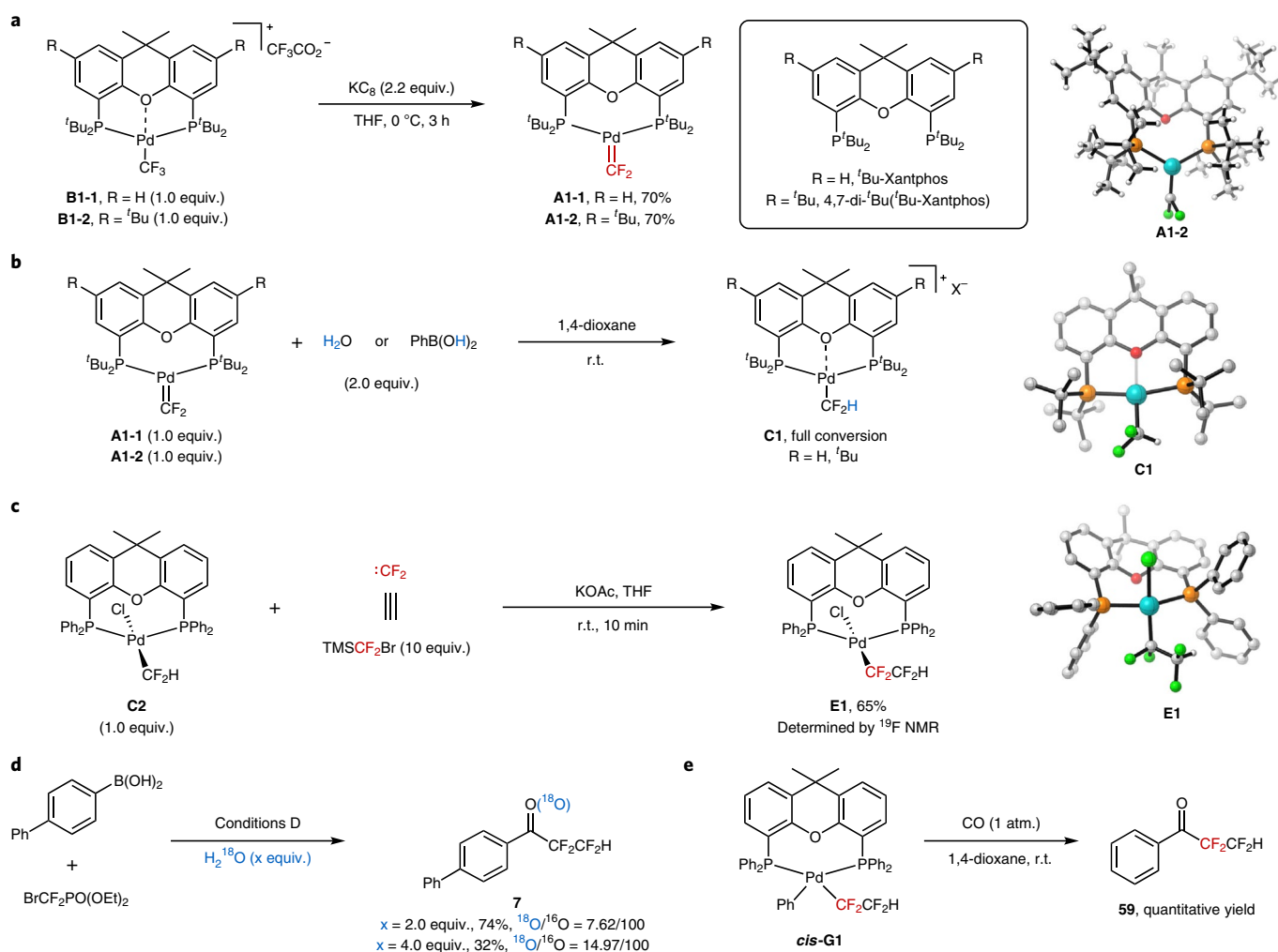
Fig. 3 | Mechanistic studies. a , Preparation of [Pd 0 ]=CF 2 complexes A1 and single-crystal X-ray structure of [Pd 0 ]=CF 2 complex A1-2 . b , Protonation of complex A1 with H 2 O or phenylboronic acid and single-crystal X-ray structure of difluoromethyl-palladium complex C1 . The anions are not shown. c , Investigation of CF 2 elongation and the single-crystal X-ray structure of tetrafluoroethyl palladium complex E1 . d , 18 O-labelling of compound 7 . A twofold loading amount of H 2 18 O almost doubled the ratio of 18 O-labelled 7 , indicating that the CO to form the tetrafluoroethyl aryl ketones is probably derived from the hydrolysis of [Pd II ]=CF 2 . e , Reaction of cis - G1 with CO. This reaction proceeded smoothly at room temperature to give the carbonylation product in quantitative yield, whereas the reaction of palladium complex E1 with CO failed to provide the fluoroacyl palladium complex (Supplementary Fig. 7). These results suggest that the carbonylation step occurs after the transmetalation of complex E1 . X denotes hydroxyl or other oxygen anions. Colour code: grey, carbon; white, hydrogen; blue, palladium; orange, phosphorus; red, oxygen; green, fluorine.
