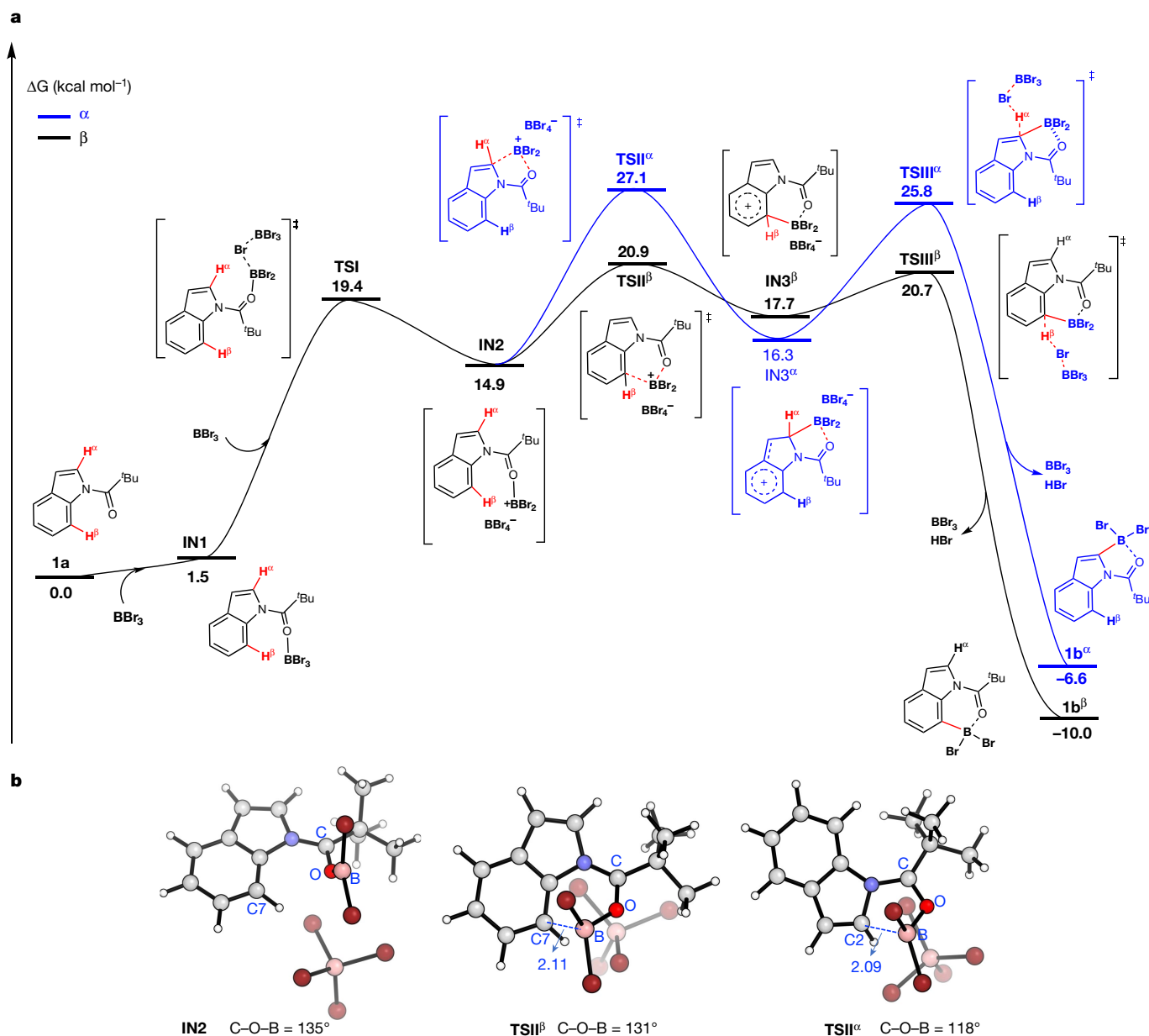
Fig. 4 | DFT calculations for the reaction of 1a with \text{BBr}_3 . a , Free energy profiles for the C–H borylation of indole 1a . b , Optimized structures of IN2 , TSII α (292i cm -1 ) and TSII β (287i cm -1 ). Bond lengths are in Å.
