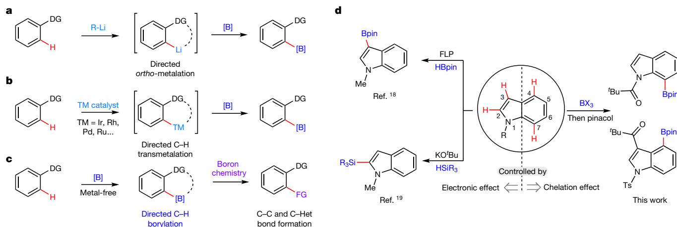
Fig. 1 | Strategies for directed C–H bond borylation. a , Directed ortho -metalation. b , Transition-metal-catalysed C–H borylation. c , Metal-free directed C–H borylation. d , Transition-metal-free site-selective C–H
