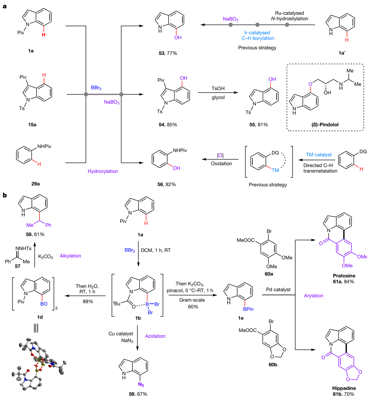
Fig. 3 | Applications of the metal-free directed C–H borylation strategy. a , Directed C–H hydroxylation mediated by boron species. b , Cascade C–H borylation/C–C and C–Het bond formation.
