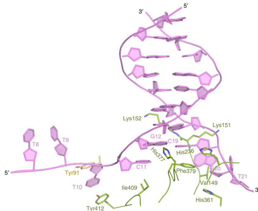
Fig. 2 Interaction of BaPif1 with forked dsDNA. Residue in brown belongs to BaPif1 A , residues in green belong to BaPif1 B and nucleotides of the forked dsDNA are in violet. Tyr91 A and Tyr412 B stack against T10. The first base pair (C11–G20) of the dsDNA is broken and C11 is stacked on one side by Ile409 B and on another side by the subsequent nucleotide G12. The other nucleotide, G20 of the broken base pair is stabilized by Val149 B and His361 B . The main chain of Lys151 B –Lys152 B anchor the phosphate backbone of the 3′ arm. A trio of residues, Phe379 B , His236 B and His377 B interact with the G12–C19 base pair of the dsDNA.
