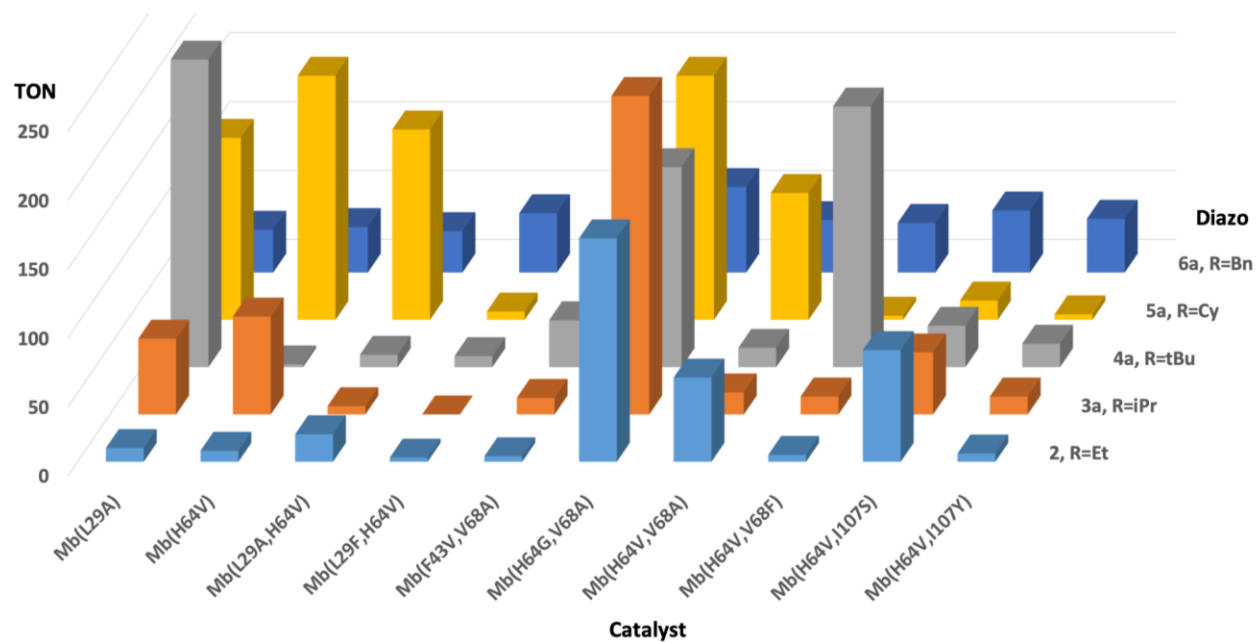
Supplementary Figure S2. Catalytic activity (turnover numbers, based on GC conversion) of selected engineered myoglobin variants in the carbene N-H insertion with benzylamine 1a and different diazo compounds ( 2 , 3a-6a ). Reaction conditions: 10 mM amine, 10 mM EDA, 20 \mu M enzyme, 10 mM Na 2 S 2 O 4 , 50 mM phosphate buffer (pH 8.0).
