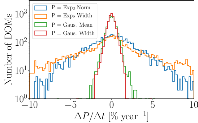
Figure 10. The change in the individual DOM fitted parameters, \Delta P , over time, \Delta t . The histogram represents the rate of change, per IceCube season, of the fitted parameter labelled in the legend.
