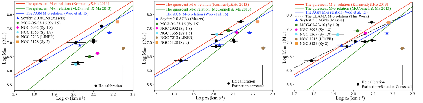
Fig. 5. Left: M_{\text{BH}}-\sigma_* relation of our sample of galaxies, where M_{\text{BH}} values are estimated using the \text{H}\alpha -based calibration. The M_{\text{BH}}-\sigma_* relation of KH13, MM13, and W15 are presented as red, green, and blue solid lines, respectively. Sy 1.8, Sy 1.9, Sy 2, and LINER galaxies are presented in different colors for visual aid. The location of the two LLAMA Seyfert 2 (NGC 4388 and NGC 5728) galaxies are shown that have megamaser M_{\text{BH}} estimates as blue triangles. In addition, we present the M_{\text{BH}} estimates of NGC 5128 obtained from stellar kinematics as an orange box (Cappellari et al. 2009). Finally, the average uncertainties on the black hole mass estimates of the LLAMA AGNs ( \sim 0.40 dex) are presented as a vertical black line in the legend to avoid confusion of data points. Middle: M_{\text{BH}}-\sigma_* relation of our sample of galaxies, where M_{\text{BH}} values are estimated using the extinction-corrected fluxes and the \text{H}\alpha calibration. Right: M_{\text{BH}}-\sigma_* relation of our sample of galaxies, where the \text{H}\alpha M_{\text{BH}} values are presented as the extinction-corrected and \sigma_* values are presented as rotation-corrected. The LLAMA M_{\text{BH}}-\sigma_* relation is presented as a black dashed line.
