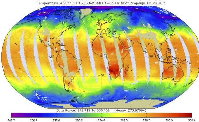
Figure 1: Level-3 temperature data in K from AIRS for the descending node at a pressure level of 850 hPa
