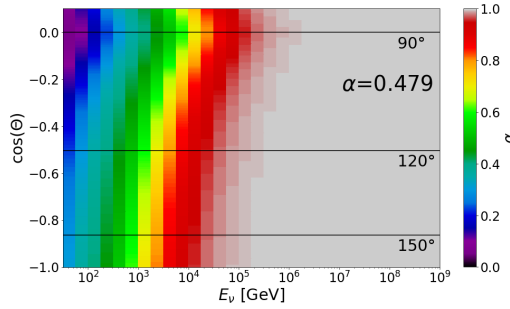
Figure 5: Calculated \alpha for the standard US atmosphere and air shower model (I)
