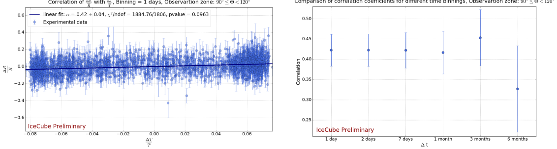
Figure 4: Correlation of atmospheric neutrino rate changes with relative changes of T_{eff} (left panel) and comparison of the correlation coefficients for several time binnings (right panel).
