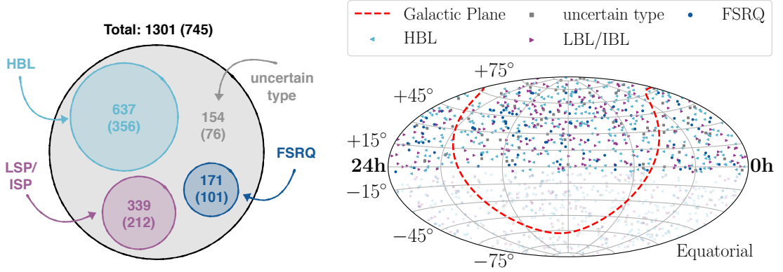
Figure 1: Left: Partition of the blazars from the 3FHL catalog into different categories. The numbers show the frequency of the respective type (numbers in brackets only take Northern hemisphere sources, \delta > -5^\circ into account). Right: Location of the 3FHL blazars. Southern hemisphere sources are shown with higher transparency.
