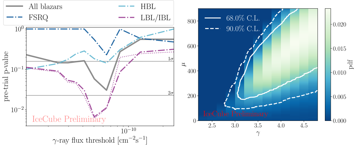
Figure 2: Left: Pre-trial p-values for blazars from the 3FHL catalog for different gamma-ray flux thresholds. Right: Confidence level contours on the mean number of signal events \mu and the spectral index \gamma for the subsample of LBL and IBLs which show the highest significance in this analysis.
