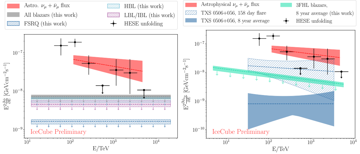
Figure 3: Left: 90 % C.L. upper limits for blazar populations from the 3FHL catalog for \gamma = 2 . The dark-shaded bands illustrate the 1\sigma central band which arise from different weighting schemes for the individual sources. The energy ranges mark the 90 % region where IceCube has the highest exclusion power for the particular model. The best fit to the astrophysical diffuse muon neutrino flux \phi_{\nu_\mu + \bar{\nu}_\mu}^{\text{astro}} from [10, 11] including the 68 % C.L. contours is displayed in red. Right: 90 % C.L. limit on the average flux of all blazars from the 3FHL catalog for \gamma = 2.19 . The blue shaded band shows the 68 % C.L. band for the average muon neutrino flux of TXS, assuming that TXS 0506+056 is a steady neutrino source over \sim 8 years of measurement. The dashed band represents the average flux of this blazar during the 158 d flaring period in 2014/2015. The data for both bands are taken from [2]. Note that the HESE spectrum as well as the diffuse muon neutrino flux are integrated over the northern hemisphere
