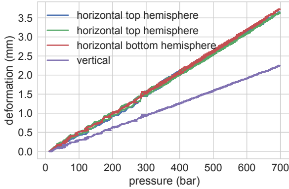
Figure 5: Horizontal and vertical (violet line) shrinkage of an mDOM pressure vessel as function of external pressure in a hyperbaric chamber. The horizontal deformation was measured separately in the upper (two sensors, blue and green lines, partially hidden) and lower ( red line) vessel half.
