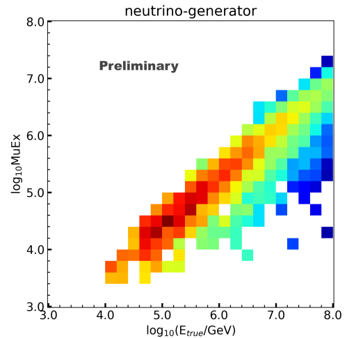
Figure 2: Relation between MuEx, the muon energy proxy used in this analysis and the primary neutrino energy for an astrophysical flux.
