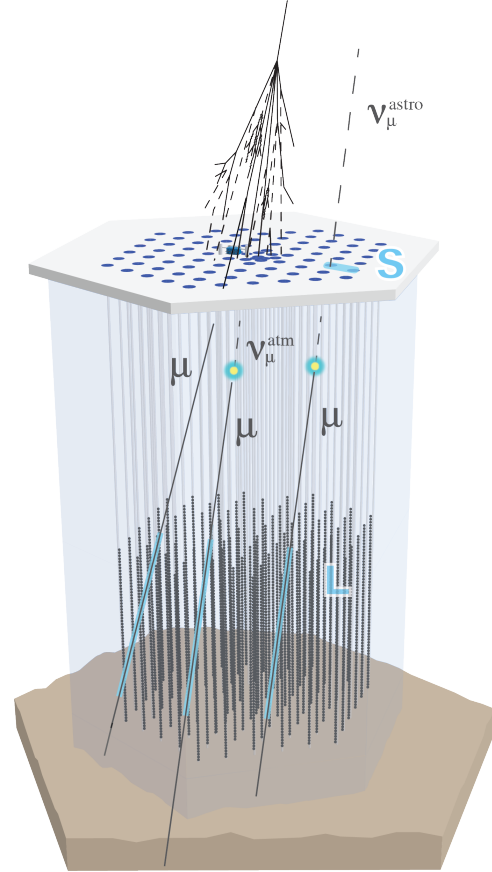
Figure 1: Illustration of the containment cuts used to select events for this analysis: track length L \geq 800 m and side distance S \geq 60 m. Additional quality cuts are applied as described in the text.
