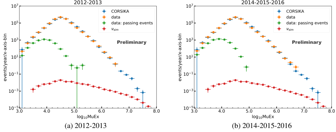
Figure 5: Number of events per year and bin as a function of muon energy proxy for CORSIKA, simulated neutrinos, and data (2012-2013 and 2014-2015-2016) before and after the veto cuts.
