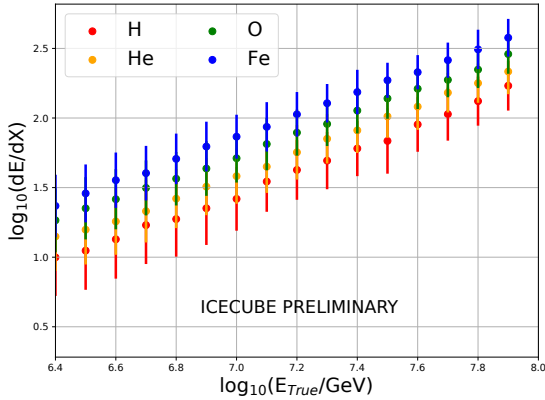
Figure 3: Mean and standard deviation of reconstructed \log_{10}(dE/dX_{1500\text{m}}) in IceCube as a function of energy for different primaries.
