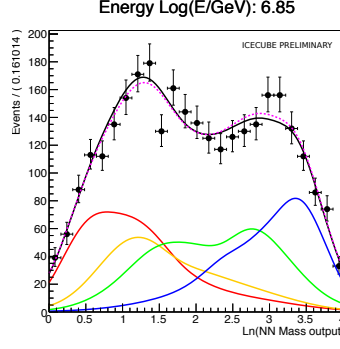
Figure 6: Example fast Monte Carlo data set from the improved analysis from the maximum mixing scenario of the four elementary groups (Fraction: 25%:25%:25%:25%) in the energy bin \log_{10}(E/\text{GeV})=6.8 -6.9 with in total 3000 MC events. The generator PDF is shown as a solid black line, the fitted PDF is shown as a dashed magenta line. The corresponding weighted elementary group PDF are shown in red for H, yellow for He, green for O and blue for Fe.
