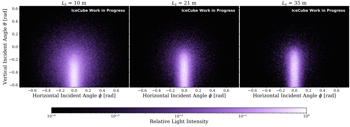
Figure 5: Images simulated using photon propagation software [10]. These images represent different effective scattering lengths ( L_s ). The light intensity in each image was scaled so that the maximum intensity is 1.
