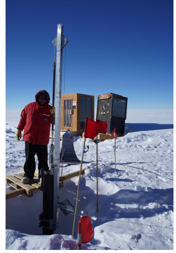
Figure 2: A photo of the device taken at the SPICEcore hole immediately prior to deployment.
