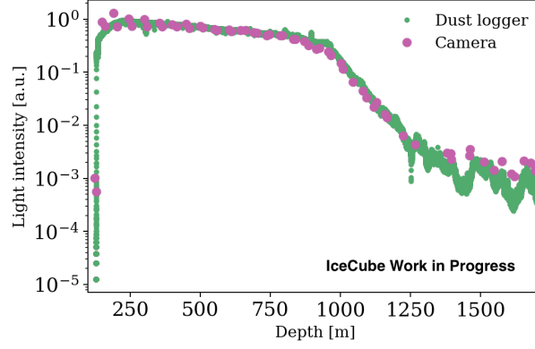
Figure 4: The intensity of back-scattered light measured by the cameras and the dust logger is shown. The light intensity for the cameras is computed as the average pixel brightness, scaled to 1 s exposure time and shown as a function of depth. The dust logger points are scaled to match the data from the camera.
