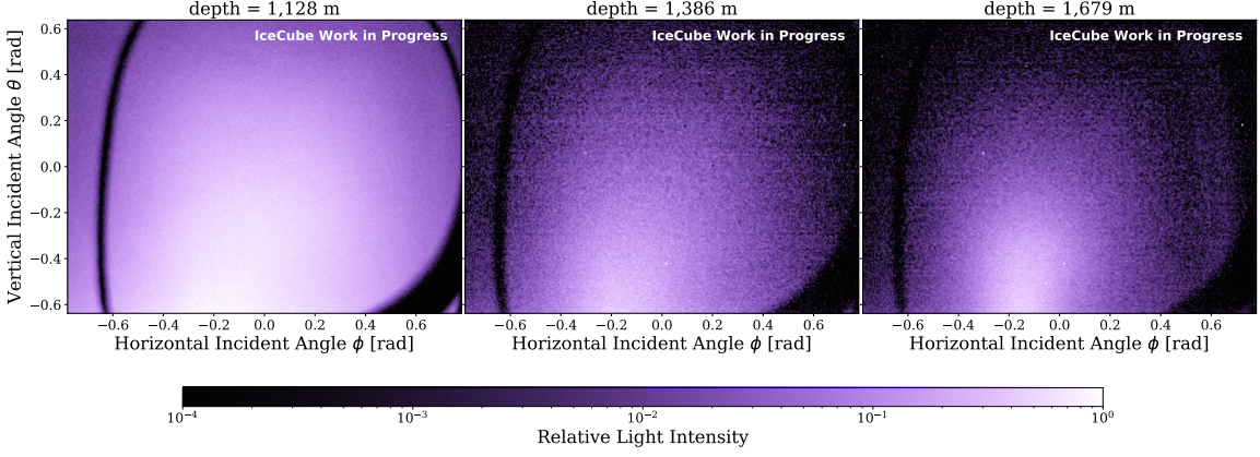
Figure 3: Images taken at different depths using one of the three cameras. The light incident angles are calculated based on the positions of pixels in each image and the Field-of-View of the camera. The dark areas that cut sharply into the light distribution stem from a harness that was used to hold the device. The light intensity in each image was scaled so that the maximum intensity is 1. The camera settings for capturing these images were the same.
