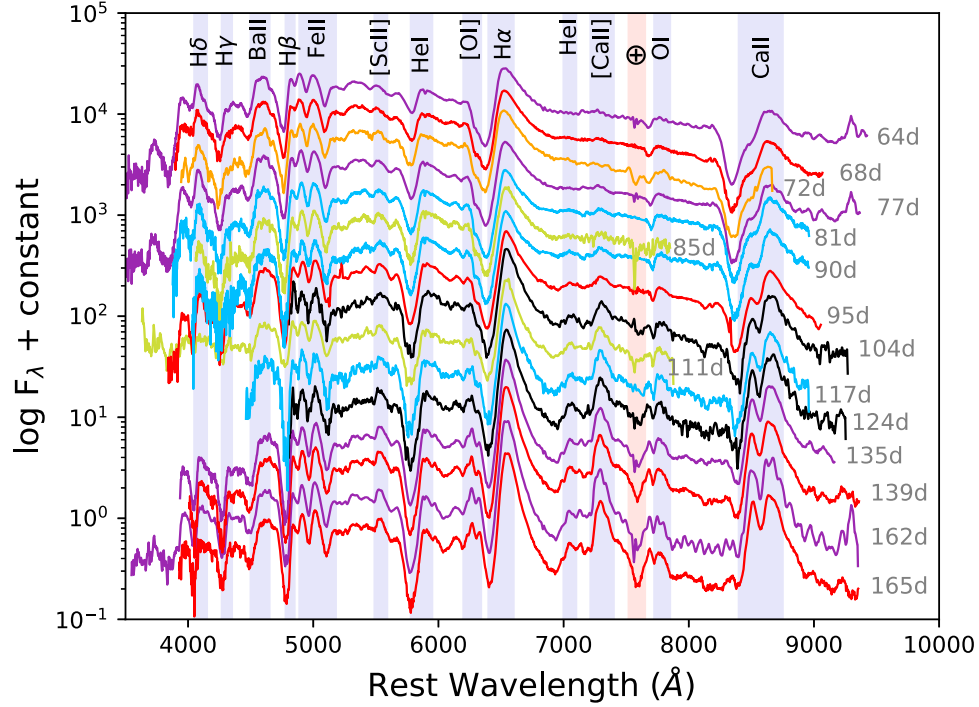
Figure 12. Same as Figure 10, but for 64–165 days after explosion.
