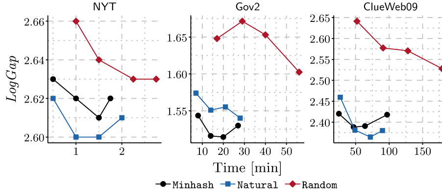
Fig. 1: \text{LogGap} cost of the three different input orderings after running BP as the number of iterations increases.
