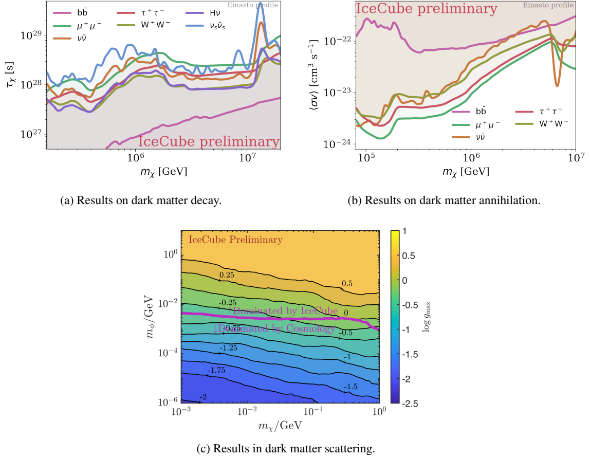
Figure 2: Constraints for dark matter decay, annihilation, and scattering with neutrinos. The three main results of this analysis are shown as a function of the dark matter mass, m_\chi . (a): Constraints on dark matter lifetime for different assumed decay modes shown as different line colors. (b): Constraints on the dark matter annihilation cross section to different standard model particles. (c): Constraints on the neutrino dark matter cross section via looking for signatures of neutrino scattering. In this analysis we assume the dark matter is a fermion and the interaction mediator, \phi , is a vector. The vertical axis shows the assumed mediator mass, m_\phi , and the color scale gives the maximum allowed log of the coupling. The magenta line signals the regions where cosmological observations are more constraining and where this analysis constraints are dominant.
