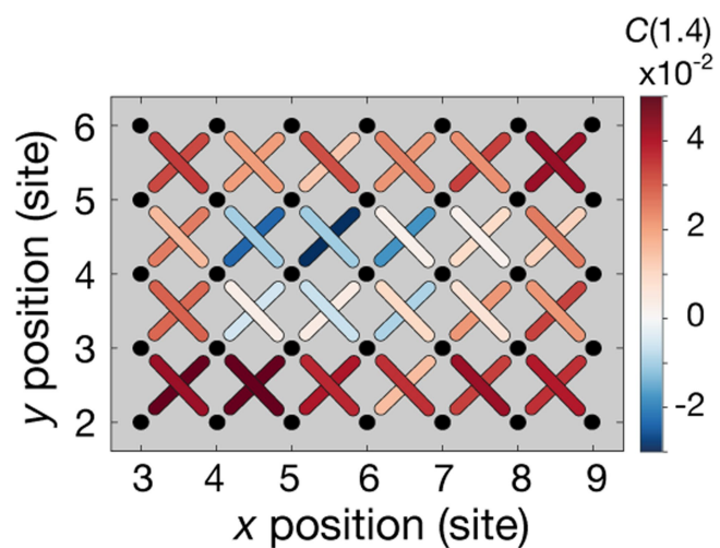
Extended Data Fig. 8 | Diagonal two-point spin correlations. Spin correlations in the central region (see lattice site positions in Fig. 2), represented by bonds connecting the two sites (black dots). At the centre, a clear reduction of correlations from the positive antiferromagnetic background value is visible. In the area of highest doublon density, correlations even flip sign and become negative.
