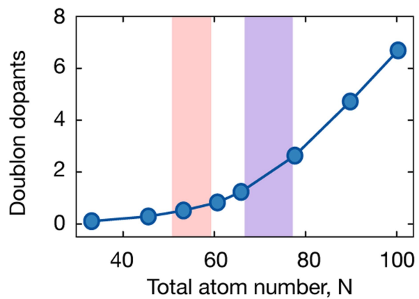
Extended Data Fig. 3 | Doping calibration. a, b , When scanning our final evaporation parameters, we measured the fraction of double occupations ( a ) and the number of doped doublons ( b ; excluding doublon-hole fluctuations) in the system as a function of the mean total atom number, N . Statistical error bars are smaller than the marker size. Pinned doublon measurements were taken in an undoped system (pink bar). For the mobile doublon dataset, settings for weak doping were used (purple bar). The bar width represents the standard deviation, obtained from atom number fluctuations.
