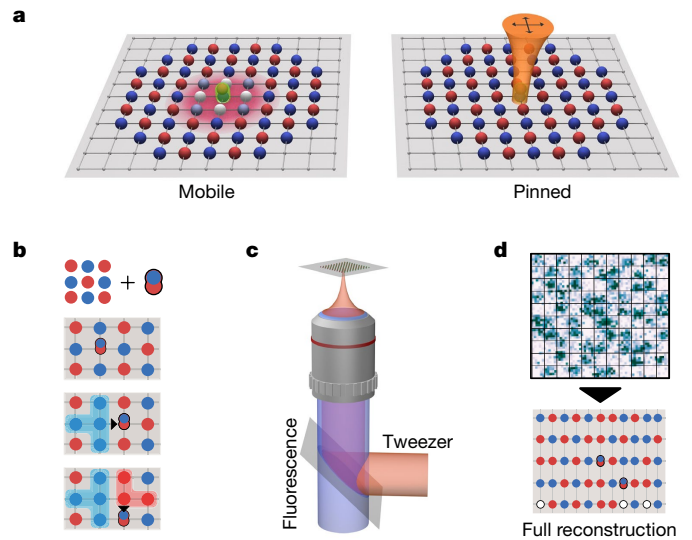
Fig. 1 | Mobile and immobile dopants with ultracold atoms. a , We experimentally study two-dimensional Fermi–Hubbard systems containing fermionic spin-up and spin-down particles (red and blue spheres, respectively), with mobile (left) or immobile (right) doublons (green), using a quantum gas microscope. In the mobile case, antiferromagnetic correlations close to the doublon are diminished (pink shading). This effect is absent in the immobile case, when the doublon is pinned with a focused attractive laser beam (orange). b , The hopping of a doublon (black arrow) in the antiferromagnetic background of the Fermi–Hubbard model around half-filling leads to a distorted spin order. With increasing delocalization, antiferromagnetically aligned spin pairs are turned into ferromagnetic ones (red and blue shading, highlighting ferromagnetic regions of different magnetization). As a consequence of this competition, theoretical and experimental evidence points towards polaron formation (see text). c , To create immobile localized doublons, we focus an attractive laser beam (orange) onto a single lattice site through the microscope, which collimates the fluorescence light (blue) for detection. d , Each captured image corresponds to a projected many-body quantum state. By employing our local Stern–Gerlach technique, we fully resolve spin and density (including holes, represented by white circles), enabling local investigation of the spin environment around doublons. As indicated in the reconstructed image, the Fermi–Hubbard model is implemented with equal tunnelling amplitudes, t_y = t_x , but unequal lattice spacings, a_y = 2a_x , to allow spin-resolved detection.
