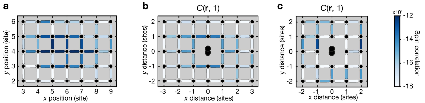
Extended Data Fig. 9 | NN correlations around mobile or pinned doublons. a , Two-point NN correlations in the central region for the mobile doublon setting, represented by colored bonds between lattice sites (black dots). b , NN spin correlations as a function of distance from mobile
