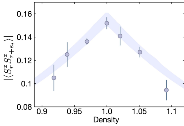
Extended Data Fig. 5 | Temperature estimation. Two-point NN spin correlations as a function of binned density. Error bars denote one s.e.m. Upper (lower) values of the purple band correspond to temperatures of T/t = 0.43 (0.46) in numerical linked-cluster expansions at U/t = 13 .
