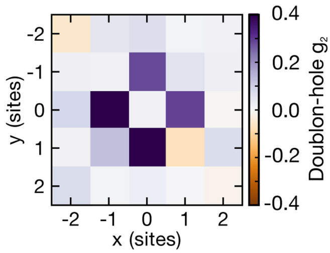
Extended Data Fig. 1 | Doublon-hole correlation. Two-point correlation function g_2 between double occupations and holes, showing a strong bunching effect at NN distances. This motivates us to neglect double occupations with holes as NNs in the analysis of mobile doublons.
