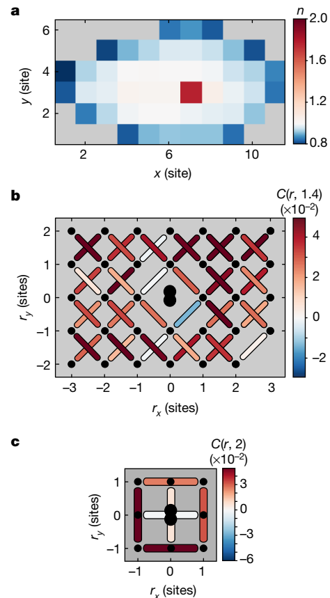
Fig. 3 | Spin correlations around trapped doublons. a , Density distribution for pinned doublons. An attractive laser beam (tweezer; 702 nm) focused on a single site artificially increases the density in an undoped system at a specific site to about 1.77(1). b , Diagonal spin correlations around doublons trapped in the tweezer. The sign-flipped spin distortion vanishes, in contrast to the mobile case. c , NNN spin correlations across and next to pinned doublons. Although spins across the trapped doublon are uncorrelated, correlations neighbouring the trapped doublon are slightly enhanced compared to the background value (see Fig. 4c). Trapping doublons with a tweezer beam prevents the competition between kinetic and magnetic energy and suppresses polaron formation (see Fig. 1a, right).
