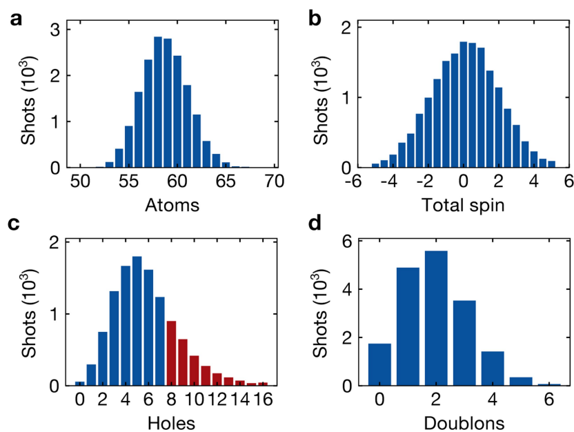
Extended Data Fig. 2 | Dataset statistics for the measurement of mobile doublons. a–c , Distribution of the number of atoms ( a ), spins ( b ) and holes ( c ) in the region with density greater than 0.7. Red bars in c indicate
