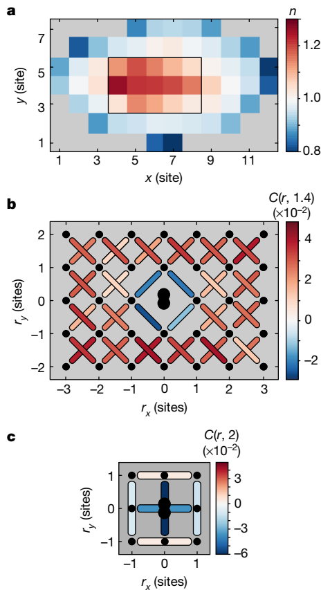
Fig. 2 | Mobile doublons dressed by local spin disturbance. a , Density ( n ) distribution for mobile doublons. In the doped region (inner black box), two doublons on average delocalize in an area of 5 \times 3 sites. b , Diagonal spin correlations, represented by bonds connecting two sites (black dots) and sorted according to their distance from doublons (double black circle at centre). Correlations are negative only in the immediate vicinity of a doublon and positive farther away. c , NNN spin correlations across and next to detected doublons. As in the case of diagonal correlations ( b ), the correlations across doublons are sign-flipped with respect to the antiferromagnetic background value. Our experimental results confirm the formation of a magnetic polaron, in which doublons are dressed by a local spin distortion (see Fig. 1a, left).
