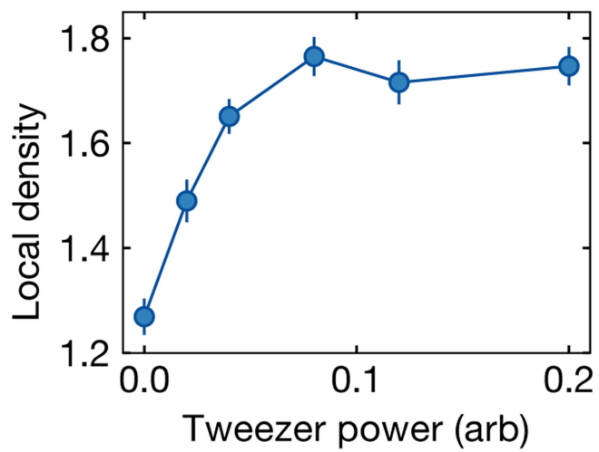
Extended Data Fig. 4 | Calibration of tweezer power. Density of the lattice site on which the tweezer is focused as a function of final tweezer power. Error bars denote one s.e.m. For the realization of pinned doublons the power was set to 0.11 (arbitrary units).
