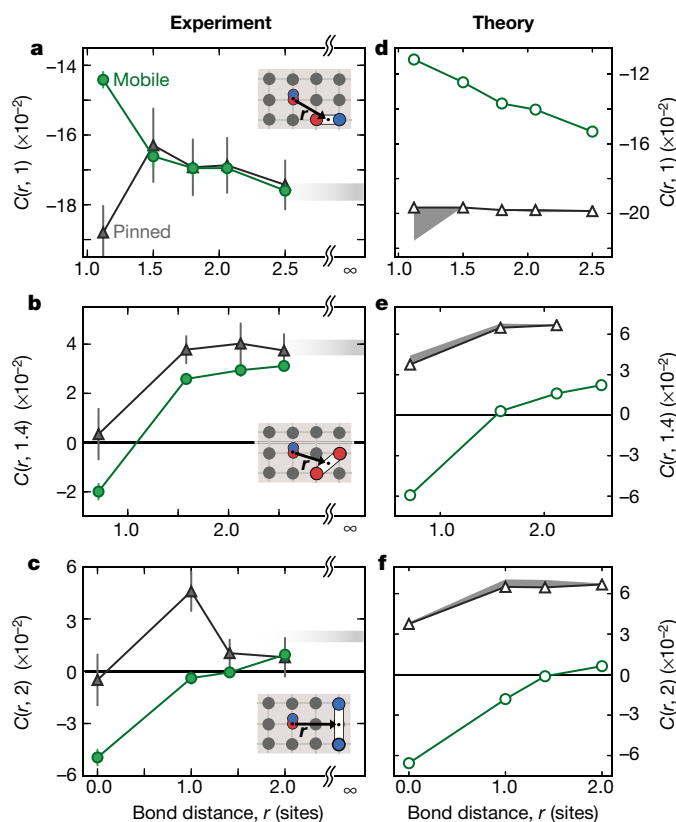
Fig. 4 | Spin correlations as a function of bond distance from doublons. a–f , Comparison between experiment ( a–c ) and numerical calculations performed using a string model for magnetic polarons and exact diagonalization of an immobile doublon in the t – J model ( d–f ). NN ( a , d ), diagonal ( b , e ) and NNN ( c , f ) spin correlations as a function of bond distance from mobile (green) or immobile (black) doublons. The insets show one exemplary bond (white) between two particles and its distance r from a doublon (double circle). Error bars denote one standard error of the mean (s.e.m.). For mobile doublons, diagonal and NNN correlations within an average bond distance of one lattice site are sign-flipped with respect to the antiferromagnetic background. Correlations quickly recover at larger distances to a value approaching the undoped antiferromagnetic value, represented by the grey band at distance \infty with a width of 2 s.e.m. The string model (green in d–f ) predicts similar correlation changes with bond distance, as well as the sign reversal of diagonal and NNN correlations. For pinned doublons, the diagonal and NNN correlations at the smallest bond distance are not sign-flipped and the polaronic distortion is strongly reduced. The amplitude of the remaining weakening of the magnetic correlations is consistent with exact diagonalization calculations of a trapped doublon (black in d–f ). Owing to the finite tweezer size (see text), a slight enhancement of NN and NNN correlations around a distance of one site is visible in the experiment, which can be captured by exact diagonalization with 10% enhanced spin exchange on neighbouring sites (grey band).
