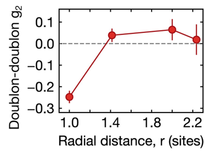
Extended Data Fig. 6 | Radially averaged doublon–doublon correlation function, g_2 . In our system, excess doublons appear anti-correlated at short distances and quickly become uncorrelated at longer distances. Error bars denote one s.e.m.
