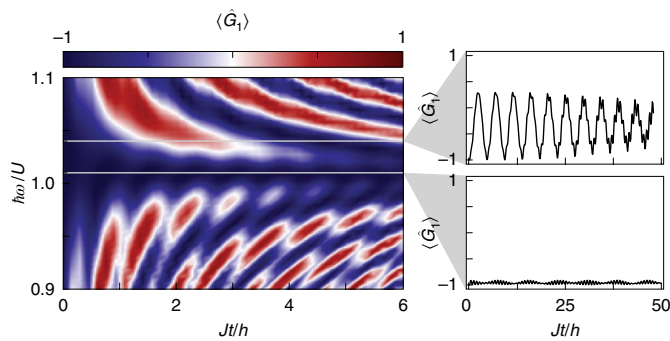
Fig. 5 | Finite-frequency corrections to the effective Floquet Hamiltonian (equation (4)). Stroboscopic dynamics of the expectation value of the local \mathbb{Z}_2 -symmetry operator \langle \hat{G}_i \rangle for |\psi_0^x\rangle , with g_1 = -1 , based on Hamiltonian (equation (3)) for different driving frequencies \omega . The panels on the right show examples of the time traces for \hbar\omega \approx 1.04U (top) and \hbar\omega = 1.01U (bottom).
