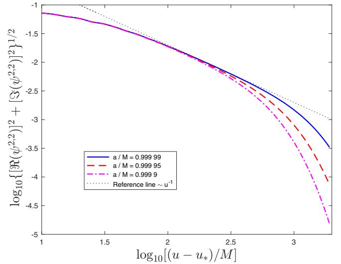
FIG. 7. Waveform amplitude plotted as a function of retarded time u at \mathcal{I}^+ for the \ell, m = 2, 2 mode of a source-free scalar field \psi for the following a/M values: a/M = 0.9999 (dash-dotted curve), 0.99995 (dashed curve), and 0.99999 (solid curve). The dotted straight line is a reference line with slope \sim u^{-1} . The parameter u_* is chosen so that the maximum of the amplitude is at u - u_* = 0 .
