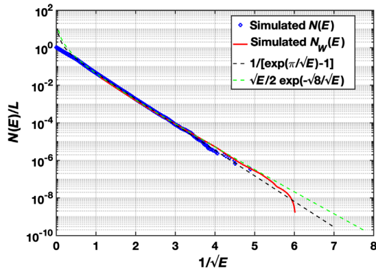
FIG. 1. Counting functions N(E) and N_W(E) computed on an interval of length L = 3 \cdot 10^6 for \rho = 1 , superimposed with the corresponding predicted analytical formulas.
