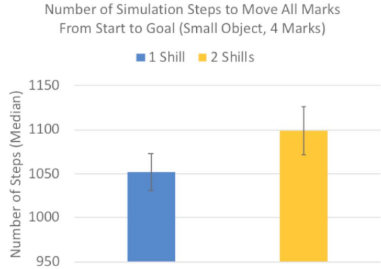
Figure 8: Chart showing how it required fewer simulation steps to shepherd four marks with 1 skill than 2 skills.
