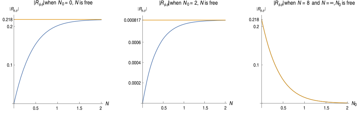
FIG. 1. The absolute value of R_{\hat{\phi}_k(\eta_1), \hat{\phi}_{-\bar{k}}(\eta_2)} . N_0 is the number of e-folds between the horizon crossing time \eta_k of the mode and \eta_1 , while N is the number of e-folds between \eta_1 and \eta_2 . Left panel: \eta_1 is chosen to be the horizon exit time for the mode, so N_0 = 0 , while N varies. The asymptotic value ( N \rightarrow \infty ) of the ratio is approached rapidly. Already at N = 2 , the ratio differs from its asymptotic value by only 8.56 \times 10^{-4} or by 0.4%. Middle panel: \eta_1 is now chosen to be 2 e-folds to the future of \eta_k , so N_0 = 2 and N is again allowed to vary. Now the asymptotic value is reached even more rapidly. For N = 2 , now the difference from the asymptotic value is reduced to 0.25%. Right panel: Now N is kept fixed and N_0 varies. The plots for N = 8 and N = \infty are indistinguishable at this resolution.
