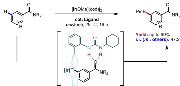
Scheme 35. Hydrogen-bonding interactions mediated by a bifunctional urea template enables a meta -selective iridium catalyzed C–H borylation of benzamides
