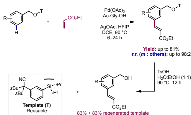
Scheme 6. Template-directed remote meta -C–H olefination of benzyl silanes
