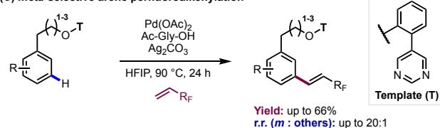
(C) meta -selective arene perfluoroalkenylation
