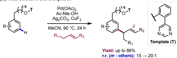
(C) meta -selective arene perfluoroalkenylation
