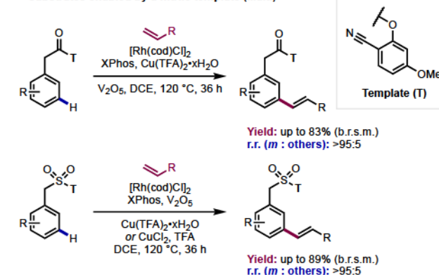
(B) Rhodium-catalyzed meta -olefination of sulfonate and phenylacetic acid substrates enabled by a nitrile template (Maiti)
