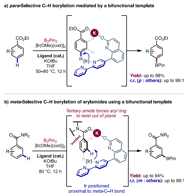
Scheme 33. Remote C–H borylation mediated by a bifunctional template anchored through potassium coordination
