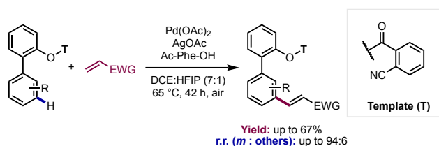
Scheme 4. Template-enabled meta -C–H olefination of biaryl phenols
