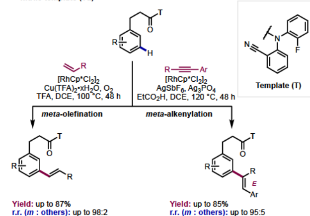
(A) Rhodium-catalyzed meta -olefination and alkenylation mediated by a nitrile template (Yu)
