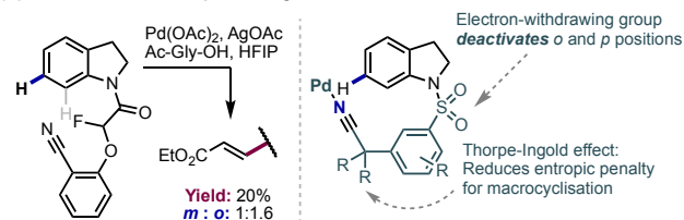
(B) meta -Functionalization of indolines enabled by sulfone-containing nitrile template
