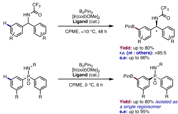
(C) Regio- and enantioselective meta -borylation enabled by ion-pairing interactions
