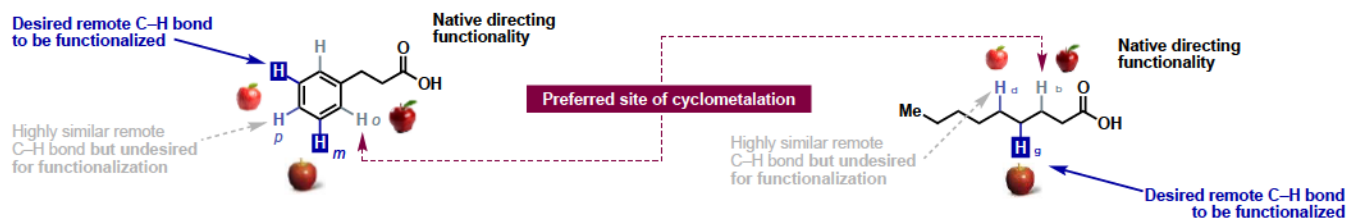
Figure 2. Central challenges in regioselective remote C–H activation and early pioneering work in this field
