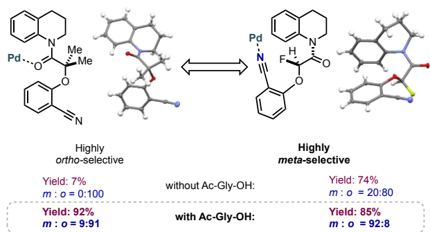
(A) Regioselectivity of C–H activation determinant on template conformation
