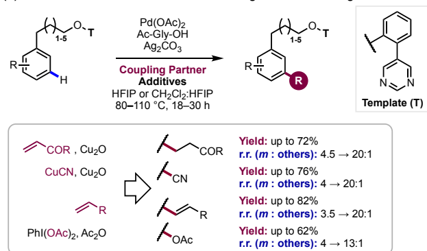
Scheme 10. meta -C–H functionalization of arenes across different linker lengths enabled by a pyrimidine template (A) meta -selective arene functionalization bearing various linker lengths
