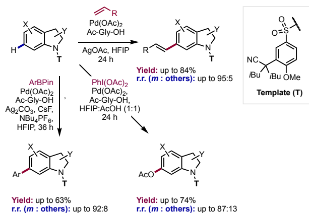
(B) meta -Functionalization of indolines enabled by sulfone-containing nitrile template
