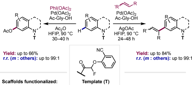
(B) Scope of meta -C–H activation: Olefination and acetoxylation
