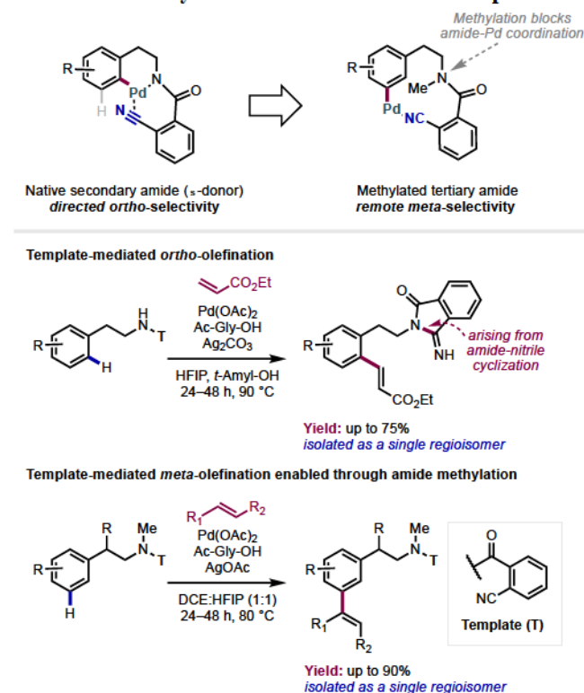
Scheme 28. A single sulfonamide-tethered nitrile template enables the divergent olefination of various N -heterocycles
