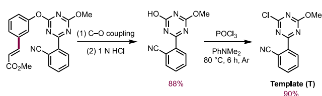
Recovery and Regeneration of Template
