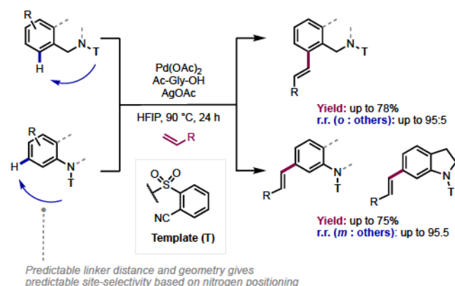
Scheme 28. A single sulfonamide-tethered nitrile template enables the divergent olefination of various N -heterocycles
