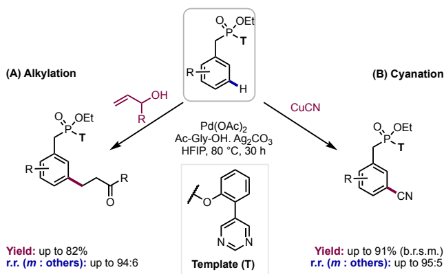
Scheme 20. meta -Deuteration of arenes bearing diverse ester-linkable functionalities enabled through a pyridine or pyrimidine-containing template
