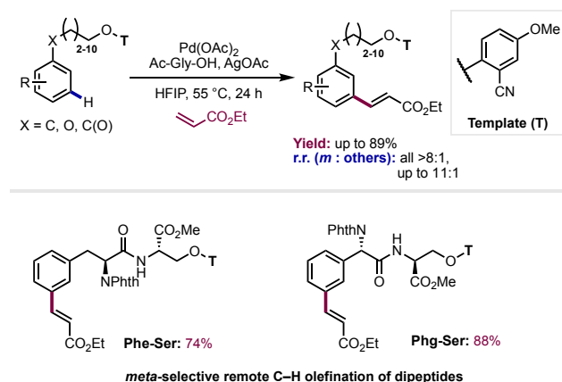
Scheme 9. Achieving selectivity in a range of distally directed meta -C–H olefination reactions for substrates containing flexible alkyl tethers
