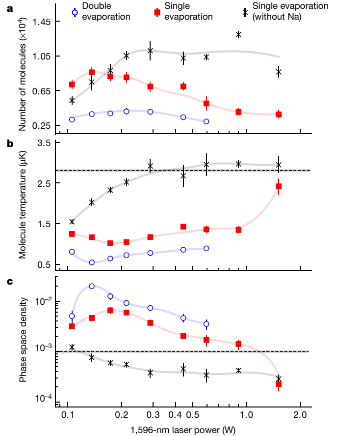
Fig. 5 | Increasing phase-space density. a–c , The number (a), temperature (b) and PSD (c) of NaLi molecules are plotted versus the power of the 1,596-nm trapping laser at the end of the forced exponential evaporation (ii) for single evaporation and (1) for double evaporation in Fig. 4). For the double evaporation, we ramp the power down to 0.06 W (2 \mu K trap depth) in (4), the lowest point that gives a molecular signal high enough for consistent temperature measurement. Single-stage evaporation to this low trap depth leads to loss of almost every molecule. The black dashed lines in b and c indicate the molecule temperature and PSD after STIRAP and removal of free atoms (shaded areas show \pm 1 error bar). This PSD corresponds to 2.6(1) \times 10^4 molecules. When Na atoms are not in the trap or when the evaporation is not performed to a sufficiently low trap depth, the PSD is lower than the initial value. This is mainly due to the molecular two-body loss. The solid curves are guides for the eye. Values and error bars are estimated as in Fig. 2 from 4–9 measurements.
