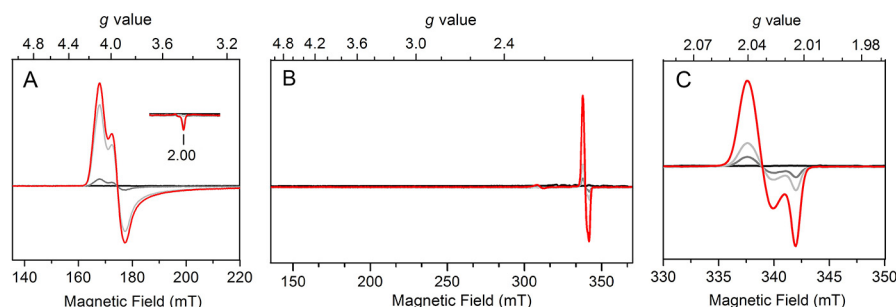
Figure 6. EPR spectra of \bullet NO addition to ADO in the absence (A) and presence (B and C) of cysteamine. \bullet NO was released by 0 (black), 0.1 (gray), 0.5 (light gray), and 2.5 (red) equiv of \bullet NO releasing agent (1 equiv of agent produces approximately 1.5 equiv of \bullet NO). A, in the absence of substrate, changes occur in the low-field (high-spin) region with increasing \bullet NO. Spectra were taken at 10 K with 50 mW microwave power. B, in the presence of substrate, changes occur in both high- and low-spin regions with increasing \bullet NO. Spectra were taken at 10 K, 1 mW. C, in the presence of substrate, changes occur in the g = 2 region with increasing \bullet NO. Spectra were taken at 50 K with 0.05 mW microwave power.
