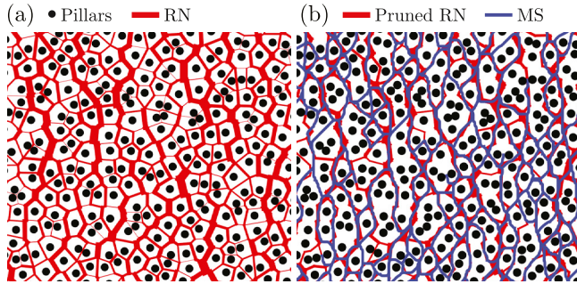
Fig. 6. Morse–Smale (MS) complex and ‘pruned’ resistor network (RN) with equivalent number of links share similar graph structure. (a) Complete RN approximation to a monodisperse porous medium. Line thickness is proportional to conductance. (b) Pruned RN with MS complex overlaid. (For interpretation of the references to color in this figure legend, the reader is referred to the web version of this article.)
