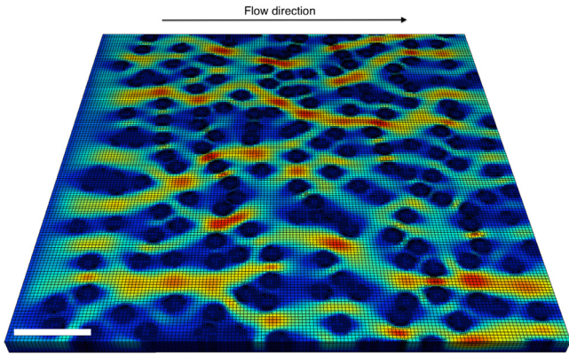
Fig. C1. Result of a 3D simulation with disorder parameter r = 1 using a local adaptive mesh (black grid lines). Scale bar 150 \mu\text{m} .
