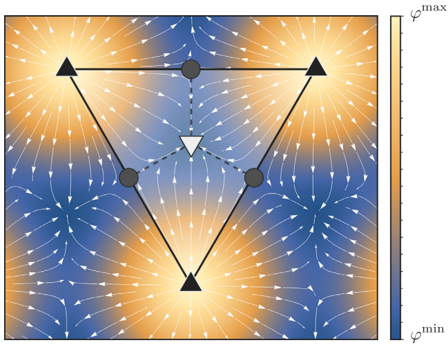
Fig. 1. Example of an ascending manifold around a single local minimum \mathbf{r}_i^{\min} (indicated by the white triangle) of a function \varphi defined on a rectangular domain \Omega . The white arrows show sample integral lines defined by Eq. (1) for various initial points \mathbf{r}_0 . The black solid lines enclose the subdomain \Omega_i^{\min} consisting of all the points that are taken by the gradient flow to the local minimum \mathbf{r}_i^{\min} (white triangle) as \tau \rightarrow \infty . The boundary \partial\Omega_i^{\min} is given by the graph (black solid lines) along which the integral lines go from maxima (black triangles) to saddle points (gray circles). The whole domain \Omega of \varphi can be partitioned uniquely in this manner, yielding a graph of connected local maxima and saddle points. The dashed black lines further partition the ascending manifold into basic cells of the Morse-Smale (MS) complex.
