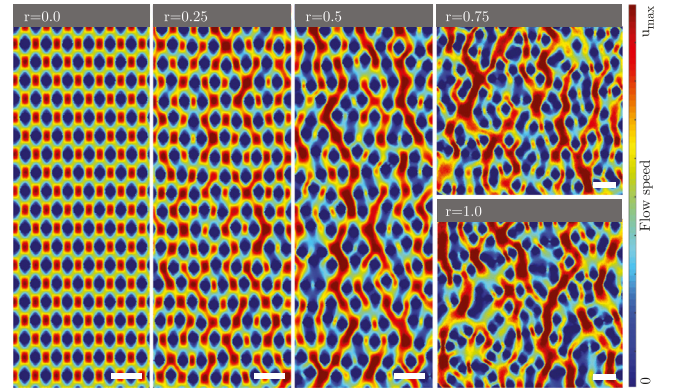
Fig. A2. Representative examples of flow speed fields measured in our experiments for different values of the disorder parameter r . Color bar: u_{\max} = 205 \mu\text{m/s} . Flow direction: from top to bottom. Scale bars 150 \mu\text{m} .
