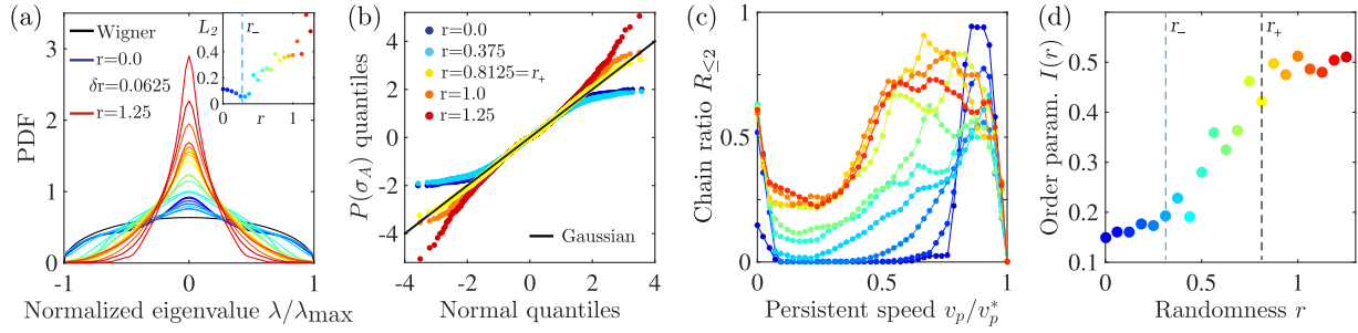
Fig. 4. Spectral properties of the Morse–Smale network ( v_p = 0.1 ) signal a disorder-induced topological phase transition towards filamentous flow structures in 2D simulations. (a) The normalized spectral density first approaches and then departs from Wigner’s semi-circle law (black line) with increasing disorder r . Inset: L_2 -distance from the Wigner law, minimum occurs at r_- \approx 0.31 . (b) The normalized quantiles of \sigma_A reveal a transition from short-tailed to long-tailed spectra at r_+ \approx 0.81 (yellow points); black line is a normal distribution. (c) The chain-link ratio R_{\leq 2} of maxima with 2 or less outgoing edges signals persistent flow filaments at high disorder r . (d) The persistence-averaged order parameter I(r) = \langle R_{\leq 2} \rangle calculated from (c), indicates the transition to filamentous flow structures with increasing r . Dashed vertical lines indicate the transition interval [r_-, r_+] , where r_- corresponds to the closest approach to the Wigner law in (a) and r_+ to the Gaussian spectral density in (b). (For interpretation of the references to colour in this figure legend, the reader is referred to the web version of this article.)
