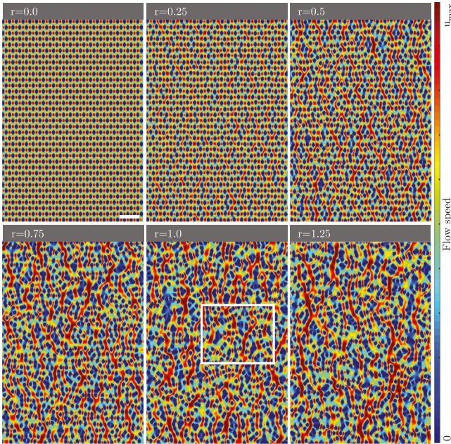
Fig. C2. Representative examples of flow fields obtained in our 2D simulations of the Brinkman model for different values of the disorder parameter r . The white rectangle indicates the subdomain shown in Fig. 1e of the Main Text. Color bar: u_{\text{max}} = 205 \mu\text{m/s} . Flow direction: from top to bottom. Scale bar 300 \mu\text{m} .
