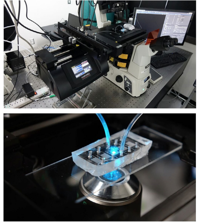
Fig. A1. Experimental setup (top) and microfluidic device (bottom). For scale, the microfluidic device is fabricated on a standard 25 \text{ mm} \times 75 \text{ mm} microscope slide.
