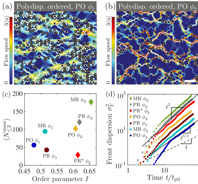
Fig. 5. Simulated flow through a polydisperse, ordered lattice at porosity \phi_1 = 0.84 (a) and porosity \phi_2 = 0.65 (b). Scale bar 300 \mu\text{m} . MS complex persistence is v_p/v_p^* = 1/3 . Colorbars are capped at 3\langle u \rangle to visualize flow channels. (c) The filament order parameter I = \langle R_{<2} \rangle confirms that low porosity geometries ( \diamond ) provide more filamentous flows independent of the type of spatial disorder. (d) Front dispersion is affected by filamentous flow structures, with almost ballistic transport for low porosities, and smaller exponents \sim t^{3/2} for equally sized media at higher porosities. Diffusive transport ( \sim t ) shown for reference.
