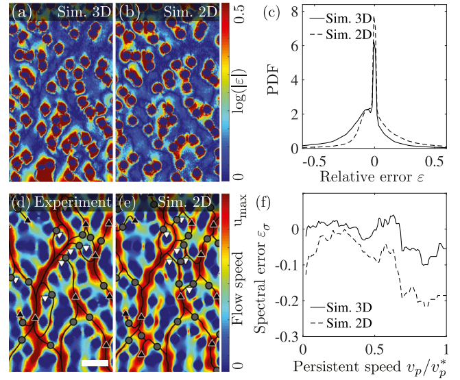
Fig. C3. Topological error estimation using Morse–Smale analysis. (a,b) The local relative error \epsilon = (v_{\text{exp}} - v_{\text{sim}})/v_{\text{exp}} between experimentally and numerically obtained flow speeds is dominated by deviations near pillar boundaries for both 3D and 2D simulations. (c) The distribution of \epsilon provides little insight into the quality of either simulation type. (d,e) Small but persistent deviations in the flow field (in units of u_{\text{max}} = 205 \mu\text{m/s} ) are made apparent by comparing the Morse–Smale graph of experiments and 2D simulations. (f) The spectral error \epsilon_\sigma defined in the text indicates that 3D simulations reproduce experimentally observed flow structures consistently better than 2D simulations. Scale bar: 150 \mu\text{m} .
