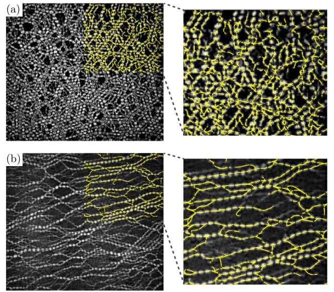
Fig. 2. Example of a MS complex showing the network encompassing the descending manifolds for stress chains in a granular medium of photoelastic disks with a diameter of 0.8 cm or 0.9 cm detailed in Ref. [24]: (a) shows biaxial compression while for (b) the compression is uniaxial. The bright areas correspond to high stress.
