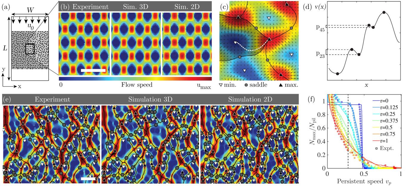
Fig. 3. Topological analysis of porous media flows. (a) Experimental and numerical porous microchannel geometry. Simulations use periodic boundary conditions in x -direction. (b) Experimental flow fields for a periodic lattice ( r = 0 ) agree with 3D and 2D simulations. Only small subdomains are shown; see Appendix C for full-size simulations. Scale bar 150 \mu\text{m} . (c) MS-complex analysis on the flow-speed field identifies persistent flow structures by connecting maxima and saddle points through integral curves (illustration; black lines separate ascending manifolds). (d) The topological relevance of a connected pair (i, j) of critical points is measured by its (flow speed) persistence p_{ij} (illustration). (e) Randomized pillar positions ( r = 1 ) favor the formation of high-speed flow field filaments. Ascending manifolds of the MS complex and extrema are shown for the persistence value v_p \approx 0.3 , corresponding to the black dashed line in (f). Scale bar 150 \mu\text{m} . (f) The number of flow speed maxima N_{\max} with persistence \geq v_p in units of u_{\max} = 205 \mu\text{m/s} , normalized by the total number of pillars N_{\text{pil}} , indicates a smooth transition in the MS complex from unperturbed ( r = 0 ) to perturbed flow fields ( r = 1 ). Deviations between experiments ( \square ) and simulations (solid lines) indicate that measurement noise dominates below v_p \approx 0.2 .
