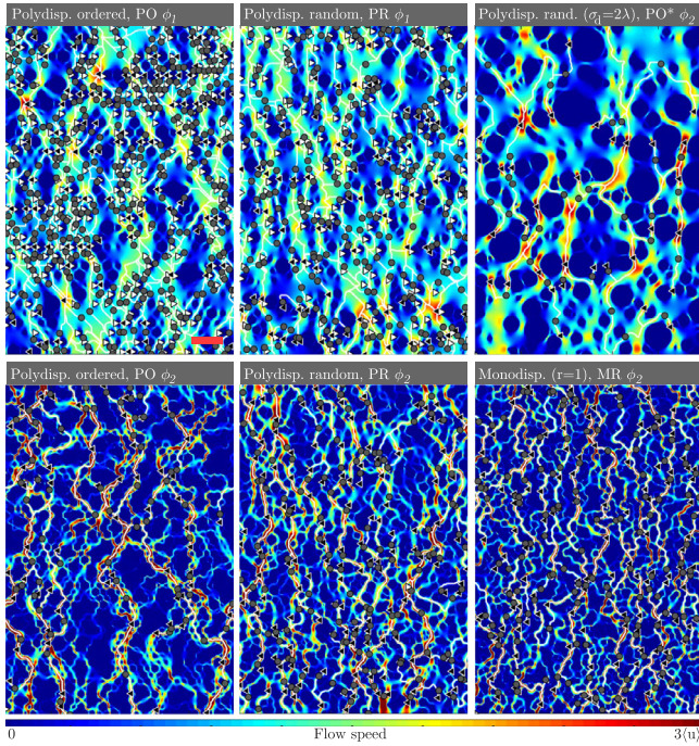
Fig. D1. Simulated flow through porous media at porosities \phi_1 = 0.84 and \phi_2 = 0.65 for polydisperse ordered (PO), polydisperse random (PR, PR*) and monodisperse media with r = 1.0 (MR). Lower porosities ( \phi_2 , higher pillar density) favor the formation of filaments and dead zones for all randomizations considered. For improved visualization of channels, colorbars are capped at 3\langle u \rangle , where \langle u \rangle is the average fluid speed in the fluid domain. Scale bar 300 \mu\text{m} .
