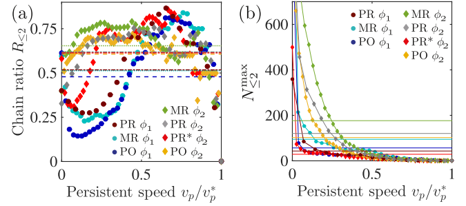
Fig. D2. (a) Flow through porous media at low porosities ( \phi_2 ) leads to larger filament chain ratios R_{\leq 2} , with small dependence on the type of random media (MR: monodisperse random, PO: polydisperse ordered, PR: polydisperse random, PR* polydisperse random with larger pillar size fluctuations). (b) The graph complexity, measured by the number of maxima forming filament chains, N_{\leq 2}^{\max} for a given persistence v_p , generally increases with lower porosity, as indicated by the averages \langle N_{\leq 2}^{\max} \rangle over 0 \leq v_p \leq v_p^* (horizontal lines).
