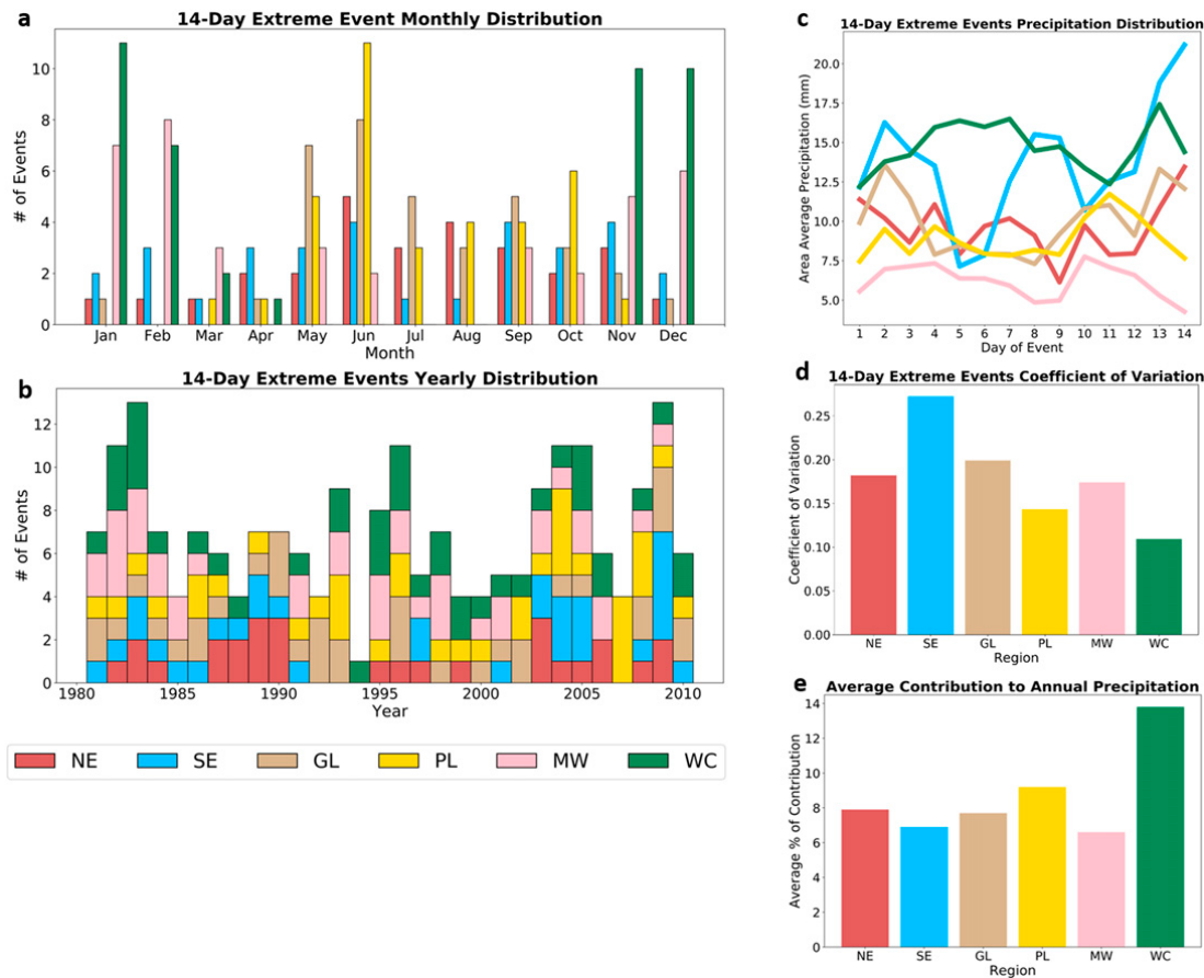
FIG. 2. Various statistical comparisons of regional 14-day extreme precipitation events: (a) monthly event distribution, (b) yearly event distribution, (c) composite of the distribution of area average precipitation for each day of the event, (d) coefficient of variation (standard deviation of events/mean rainfall per day), and (e) average event contribution to the annual precipitation total in each region.
