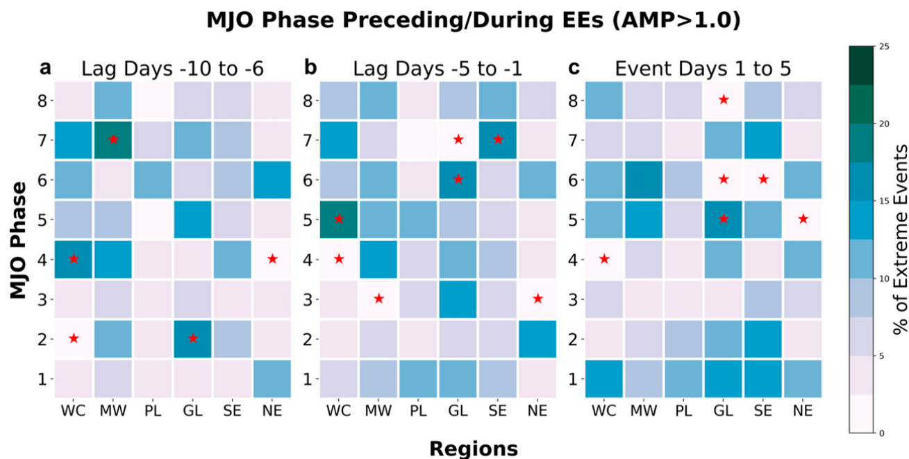
FIG. 11. Heat map of MJO phase occurrence in each region for lag windows of (a) -10 to -6 days, (b) -5 to -1 days, and (c) the first five days of the event. The daily MJO phase is based on the Wheeler and Hendon (2004) Real-time Multivariate MJO series 1 (RMM1) and 2 (RMM2). To determine the MJO phase during the 5-day windows, the mode is chosen as the window phase if it occurs in at least three of the five days. Only windows with an average 5-day amplitude of \geq 1.0 are considered. Red stars indicate that the composite percentages of occurrence for MJO phases before/during 14-day extreme precipitation events are significantly different than the mean percentage of occurrence of particular phases (roughly 7%–8%). This significance test is based on a two-tailed bootstrapping test ( p value of 0.05), with 5000 iterations and assists in identifying common and uncommon phases of the MJO before and during events.
