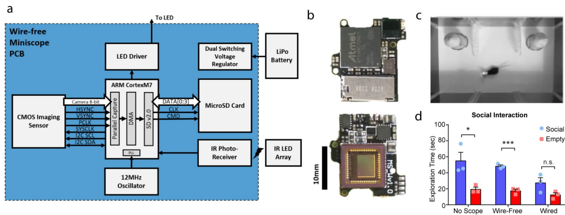
Extended Data Fig. 5 | Wire-free Miniscope design and behavior. a. Schematic of wire-free Miniscope printed circuit board (PCB). b. Picture of top and bottom of wire-free sensor board. This camera sensor board attaches to the Miniscope body, which contains all optic components. c. The wire-free Miniscope can be used to probe naturalistic behaviors including social interaction. We tested social behavior with the wire-free Miniscope compared to no Miniscope or a wired version. d. During a social interaction test mice with either no Miniscope or the wire-free Miniscope chose a social cup over an empty cup, while mice with a wired Miniscope showed no significant preference ( n = 3 per group, Unpaired t-tests, No Scope: P = 0.03 , Wire-Free: P < 0.001 , Wired: P = 0.10 ). Error bars represent 1 S.E.M. * P < 0.05 , *** P < 0.001 .
