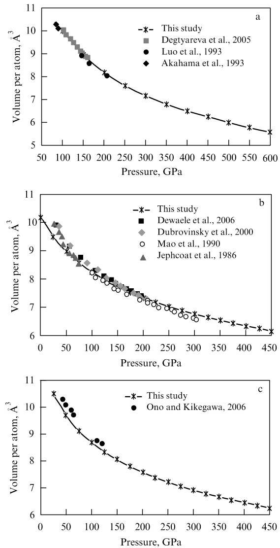
Figure 2. Comparison of the theoretical ( T = 0 K) and experimental ( T = 300 K) equations of state: (a) sulfur (experiments: Akahama et al. [11], Luo et al. [12], Degtyareva et al. [13]); (b) iron (experiments: Dewaele et al. [38], Dubrovinsky et al. [39], Mao et al. [40], Jephcoat et al. [41]), and (c) FeS (experiments: Ono and Kikegawa [42]).
