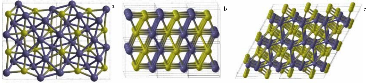
Figure 5. (Color online.) Structures of thermodynamically stable high-pressure iron sulfides found in this work: (a) Fe 2 S ( Pnma ), (b) FeS ( Pmmm ), and (c) FeS 2 ( C2/m ). Purple balls—iron atoms, and yellow balls—sulfur atoms.
