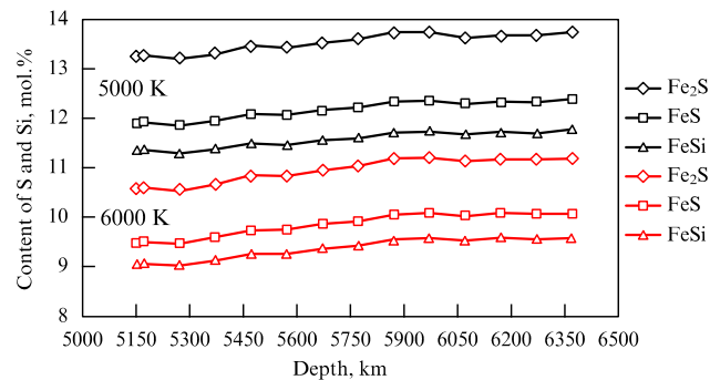
Figure 9. (Color online.) Matching molar concentration of sulfur and silicon as a function of depth in the inner core using equations of state for Fe 2 S, FeS, and FeSi. Results are shown along the 5000 K and 6000 K isotherms.
