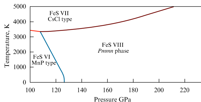
Figure 7. Phase diagram of FeS obtained in the quasiharmonic approximation.
