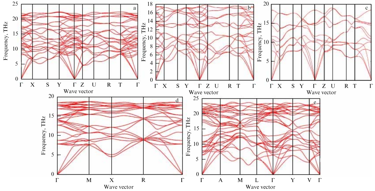
Figure 4. Phonon dispersion curves of (a) Pnma -Fe 2 S at 200 GPa, (b) Pnma -FeS at 80 GPa, (c) Pmmm -FeS at 100 GPa, (d) Pa \bar{3} -FeS 2 at 75 GPa, and (e) C2/m -FeS 2 at 250 GPa.
