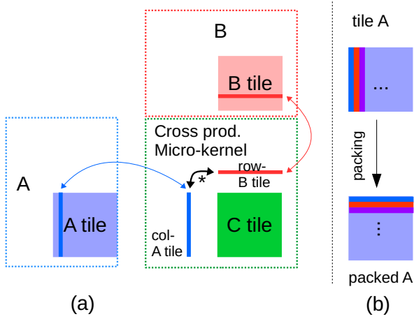
Figure 1: Data packing
