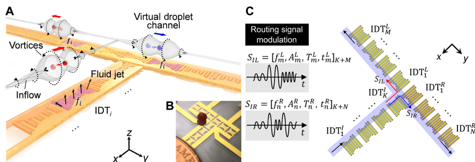
Fig. 1. ASV-based droplet manipulation. (A) Schematic showing a typical droplet processing unit. The droplets (i.e., red and blue spheres) over the transducers are guided into the center between the barrel-like ASVs (labeled as Vortices) following the recirculating inflow. These droplets are unidirectionally routed along the linear array of IDTs by shifting the sequence of working frequencies. The portions of the IDTs shaded in purple (e.g., IDT i ) indicate that they are being excited by a high-amplitude signal with frequency f_i . (B) The photo shows a bifurcated device with a particle floating above the transparent carrier oil layer. (C) The general control schematic for the droplet processing unit. The unit is composed of K + M + N interconnected IDTs [denoted as IDT k L , IDT m L , and IDT n R ( k = 1, 2, \dots, K; m = 1, 2, \dots, M; n = 1, 2, \dots, N )] with tuned working frequencies. Multitonal signals (i.e., S_{IL} or S_{IR} ) encoded with a series of different frequencies, amplitudes, durations, and initiation times (i.e., [f_m^L, A_m^L, T_m^L, t_m^L]_{K+M} or [f_n^R, A_n^R, T_n^R, t_n^R]_{K+N} ) are the excitation signals into the droplet processing unit and can direct the droplet from IDT i L to the left or right port, respectively. The blue shaded area indicates the resulting virtual bifurcated channel for droplet translation. Photo credits: Peiran Zhang, Duke University.
