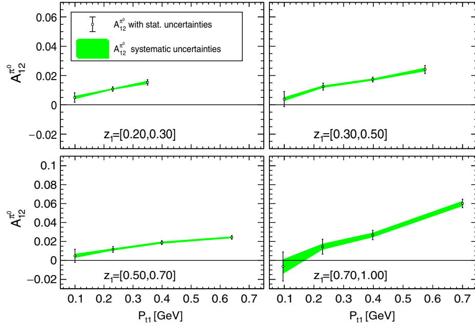
FIG. 7. Dependence of A_{12}^{\pi^0} on P_{t1} for four bins in z_1 (as labeled), integrating within the overall limits over the kinematics of the second hadron. Error bars represent statistical uncertainties while the colored bands indicate systematic uncertainties.
