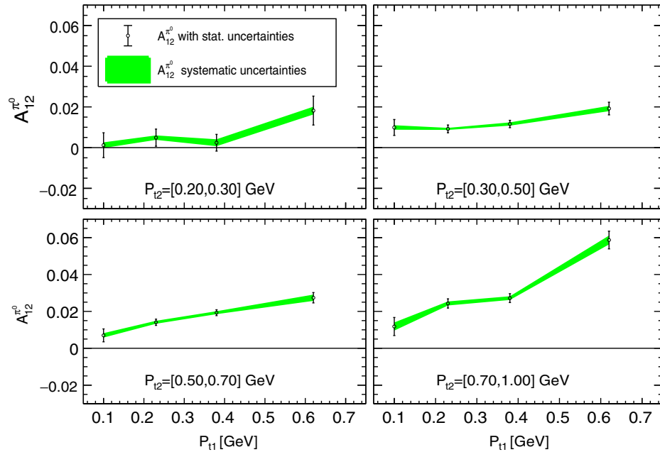
FIG. 8. Dependence of A_{12}^{\pi^0} on P_{t1} for four bins in P_{t2} (as labeled), integrating within the overall limits of [0.2, 1.0] over z . Error bars represent statistical uncertainties while the colored bands indicate systematic uncertainties.
