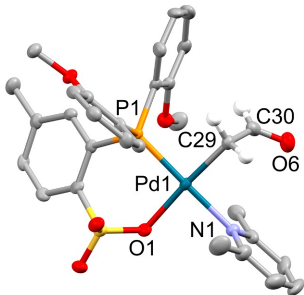
Figure 2. Molecular structure of 6 \cdot 1.5(\text{CH}_2\text{Cl}_2) . Hydrogen atoms on the \text{CH}_2\text{C}(\text{=O})\text{H} ligand were calculated using displacement parameters set to 1.2 times the isotropic equivalent of the displacement parameters of the bonded atoms. All other hydrogen atoms and the \text{CH}_2\text{Cl}_2 molecules are omitted for clarity. Bond lengths (Å) and angles ( ^\circ ): Pd1–C29 2.065(6), Pd1–N1 2.121(5), Pd1–O1 2.114(4), Pd1–P1 2.2391(16), C29–C30 1.468(9), O6–C30 1.216(8), C29–Pd1–N1 90.1(2), N1–Pd1–O1 86.45(17), C29–Pd1–P1 88.96(18), O1–Pd1–P1 94.56(12)
