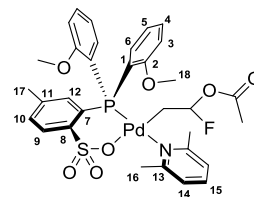
Figure 9. Atom numbering scheme for 5 .
