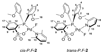
Figure 7. Atom numbering scheme for cis - P,F-2 and trans - P,F-2 .
