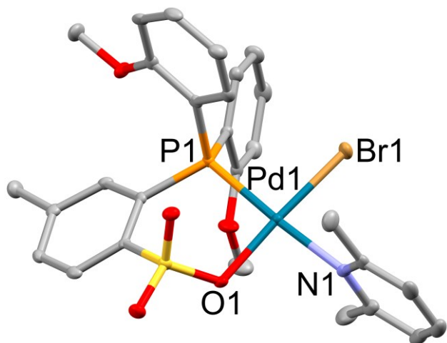
Figure 1. Molecular structure of 1 ·CH 2 Cl 2 . Hydrogen atoms and the CH 2 Cl 2 solvent molecule are omitted for clarity. Key bond lengths (Å) and angles (°): Pd1–Br1 2.3903(4), Pd1–N1 2.113(3), Pd1–O1 2.069(2), Pd1–P1 2.2483(9), Br1–Pd1–N1 88.26(7), N1–Pd1–O1 87.84(9), Br1–Pd1–P1 88.40(2), O1–Pd1–P1 95.51(6).
