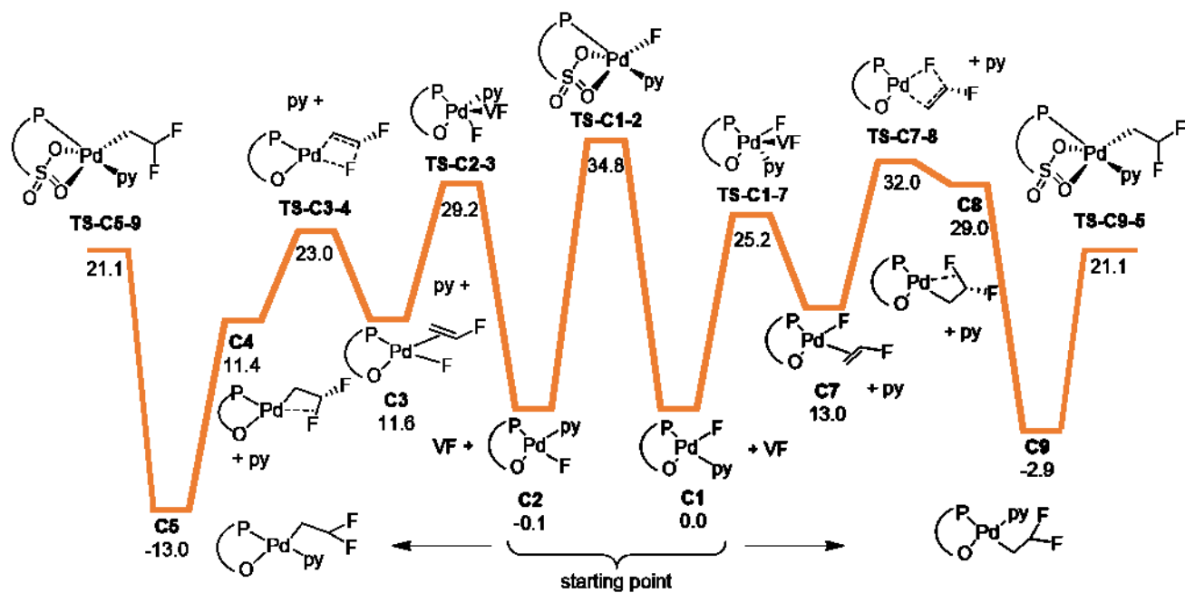
Figure 3. Computed potential energy surface for the reaction of model compounds cis - P,F -( \text{PH}_2\text{O} )PdF(py) ( C1 ) and trans - P,F -( \text{PH}_2\text{O} )PdF(py) ( C2 ) with VF. Potential energies are calculated in \text{CH}_2\text{Cl}_2 and reported in kcal/mol.
