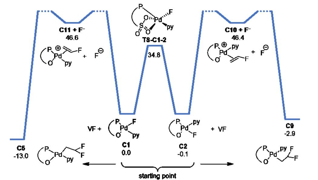
Figure 4. Potential energy surface for the reaction of cis - P,F -( PH 2 O)PdF( py ) (C1) and trans - P,F -( PH 2 O)PdF( py ) (C2) with VF via an exo attack mechanism. Potential energies are calculated in CH 2 Cl 2 and reported in kcal/mol. Transition state energies are estimated at 5 kcal/mol greater than the energies of the intermediate species C11 and C10 and fluoride.
