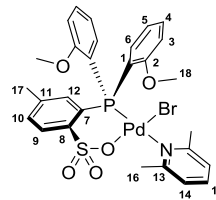
Figure 6. Atom numbering scheme for 1 .
