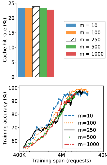
Fig. 25: Sensitivity to m , the number of generated decision samples.
