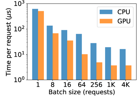
Fig. 18: Per-request neural-net processing of RL-Cache.
