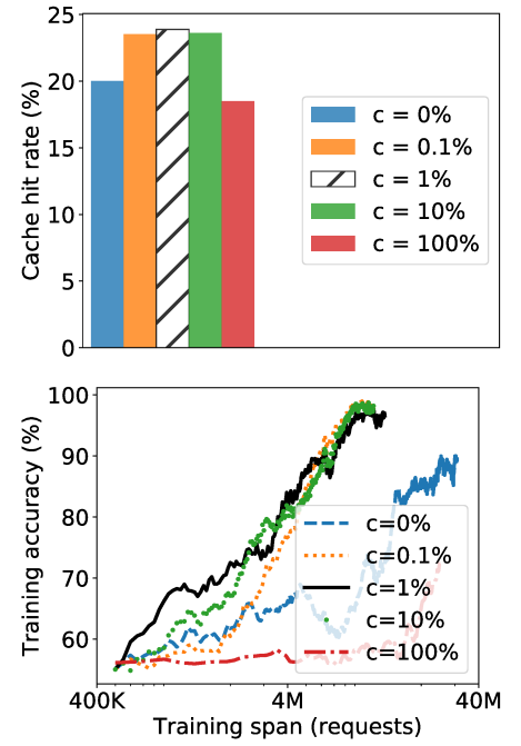
Fig. 24: Sensitivity to c , the contribution factor for the last extra request.
