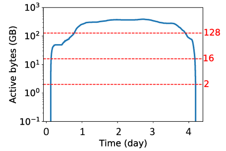
Fig. 8: Active bytes for US1-web.
