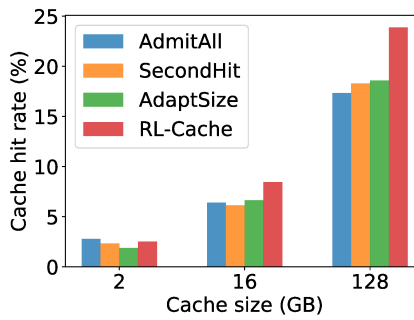
Fig. 15: Average hit rate on EU-video.
