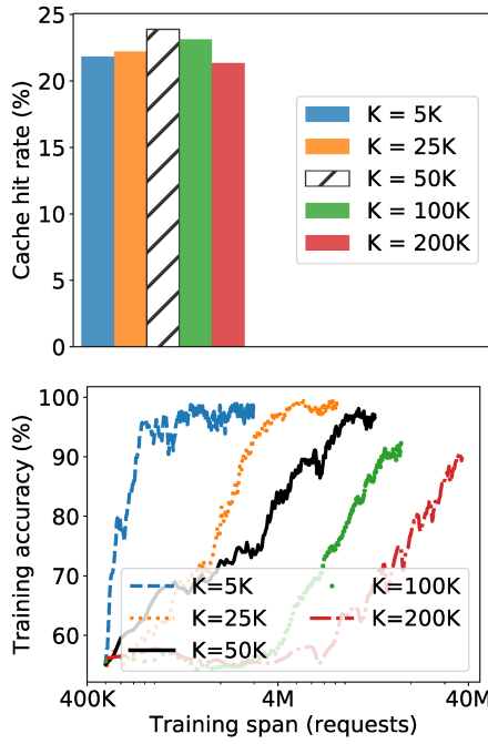
Fig. 22: Sensitivity to K , the size of a decision sample.
