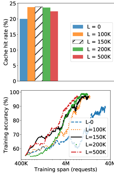
Fig. 23: Sensitivity to L , the number of extra requests per sample.
