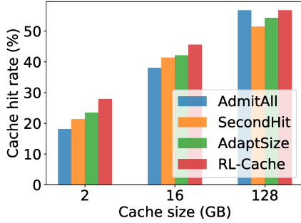
Fig. 9: Average hit rate on US1-image.
