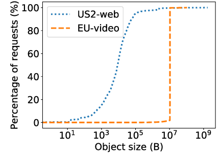
Fig. 13: Object-size distribution for the US2-web and EU-video traces.
