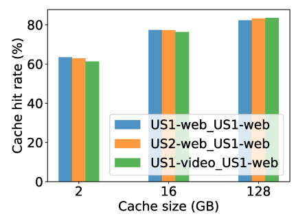
Fig. 16: Robustness within a region.
