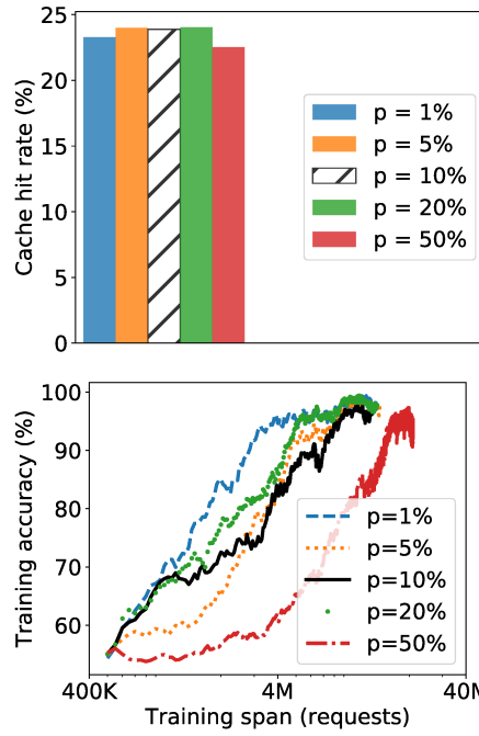
Fig. 26: Sensitivity to p , the percentage of the samples selected for learning.
