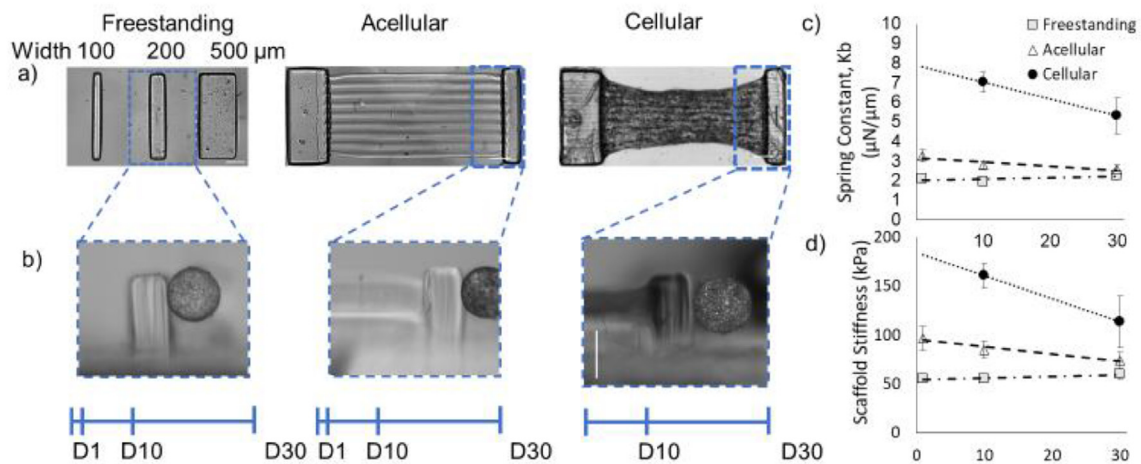
Fig. 3. Mechanical testing of NMVCM tissue. a) Mechanical testing of free standing cantilevers, acellular scaffolds and cellular scaffolds, and b) representative images of the Microsquisher pressing on each scaffold (scale bar is 500 μm). c) The spring constants of 200 μm pillars for free standing, acellular, and cellular scaffolds over 30 days. d) The calculated stiffness of each 200 μm pillar scaffolds over 30 days.
