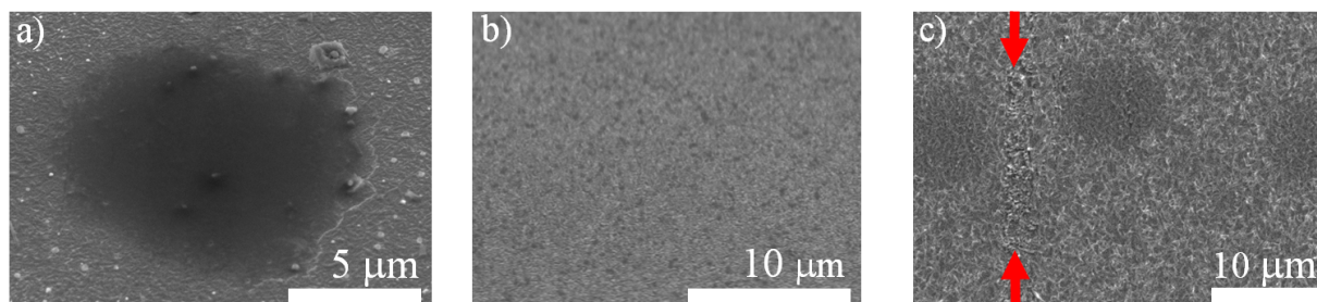
Figure 3. a) Pentacene thin film that has been reacted with maleic anhydride. b) Unreacted pentacene thin film c) Pentacene thin film reacted with maleic anhydride. Crack between red arrow lacks the surface coating and is similar of the topography of an unreacted surface
