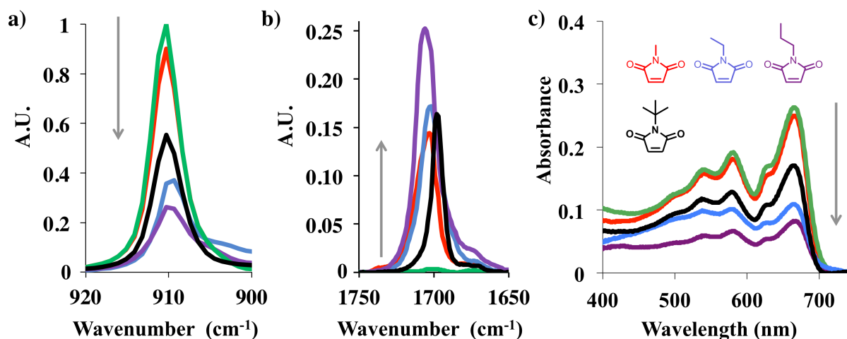
Figure 2. Reactions of thin-film pentacene (green) with N -methylmaleimide (red), N - tert -butylmaleimide (black) N -ethylmaleimide (blue), N -propylmaleimide (purple). a) pentacene consumption monitored via PM-IRRAS spectra, averages over three trials and normalized to an initial out of plane vibration value of 1. b) product formation monitored via PM-IRRAS spectra,
