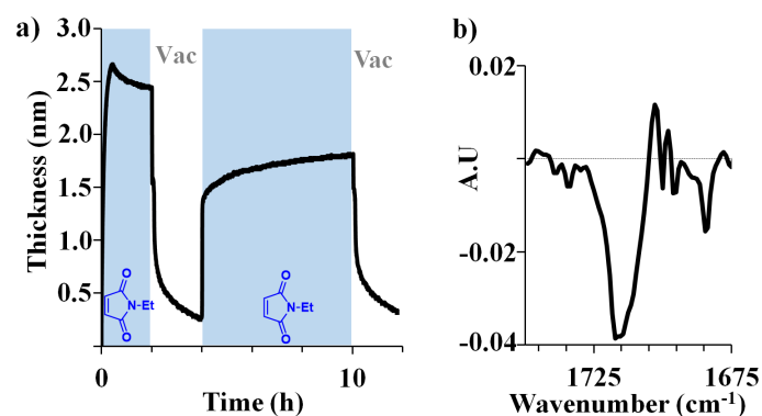
Figure 4. a) Change in the thickness of a tetracene thin film that is exposed to N-ethylmaleimide at room temperature. Blue regions show the increasing thickness due to exposure to the small molecule reactant, while white regions are time intervals when the molecular source is closed off and high vacuum is applied to the film. b) PM-IRRAS subtraction spectra of N-ethylmaleimide reacted with a pentacene thin film. The spectra taken after 6 hours of reaction at 50 °C was subtracted by the spectra taken after 30 minutes of exposure to a N 2 purge.
