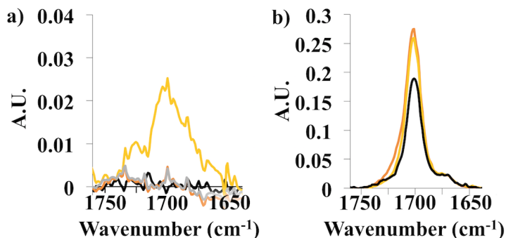
Figure 5. a) IR spectra of N -methylsuccinimide deposited onto a bare gold surface (yellow) and subjected to a N_2 purge for 5 min (orange) and then 10 min (gray). The black line is a spectra of the gold slide taken before deposition. b) PM-IRRAS spectra of N -methylsuccinimide as deposited a pentacene thin film (orange) after being subjected to a N_2 purge for 5 min (yellow), and high vacuum for 18 h (black).
