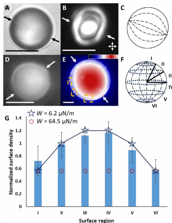
Fig. 1. Bipolar LC microparticles, experiments, and theoretical predictions.
