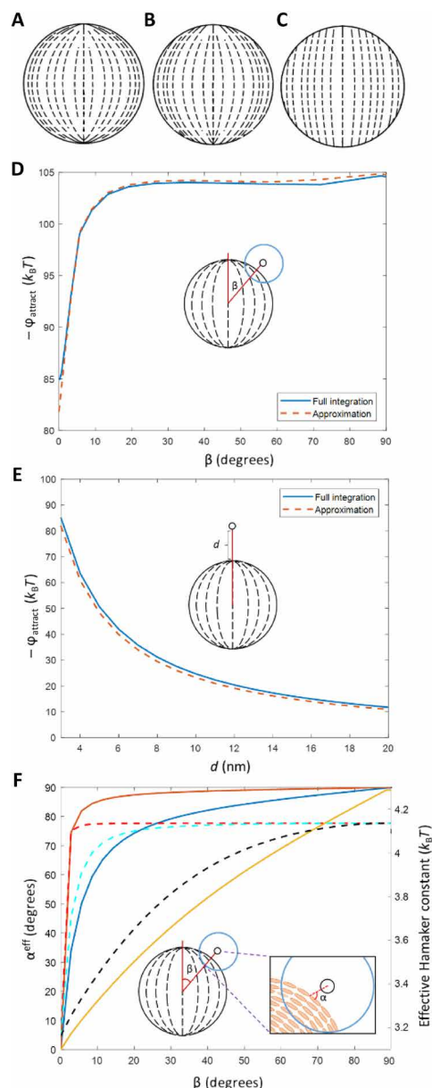
Fig. 3. Theoretical predictions of bipolar LC microparticle internal ordering and attractive interaction energies. (A to C) Director profiles in the x-z plane of a bipolar LC microparticle calculated numerically for tangential surface anchoring energies of 64.5 \mu\text{N/m} (A), 6.2 \mu\text{N/m} (B), and 0.6 \mu\text{N/m} (C). (D and E) Attractive interaction energy calculated using Eq. 1 either by (solid lines) integrating over all volume elements of a bipolar microparticle with intermediate ( W = 6.2 \mu\text{N/m} ) tangential anchoring or by (dashed lines) approximating LC ordering at the surface nearest the probe colloid as representative of the entire volume, at various angles of incidence ( \beta ) at a surface-to-surface separation, d , of 3 nm (D) and at various surface-to-surface separations above the pole ( \beta = 0^\circ ) (E). (D) Inset: Illustration showing the angle of incidence, \beta . (E) Inset: Illustration showing location of probe colloid as surface-to-surface separation is varied. (F) Calculated average director angle, \alpha^{\text{eff}} , sampled by a probe colloid as a function of \beta and a separation of 10 nm from the surface of the bipolar microparticle. (Solid lines) Results are shown for surface anchoring energies of 64.5 \mu\text{N/m} (orange), 6.2 \mu\text{N/m} (blue), and 0.6 \mu\text{N/m} (gold). The corresponding effective Hamaker constant for interaction energies calculated according to Eq. 1 (dashed lines) for surface anchoring energies of 64.5 \mu\text{N/m} (red), 6.2 \mu\text{N/m} (cyan), and 0.6 \mu\text{N/m} (black) is also shown. (F) Inset: Illustration of LC ordering near a probe colloid and the angle, \alpha , between a probe colloid and the local LC director.
