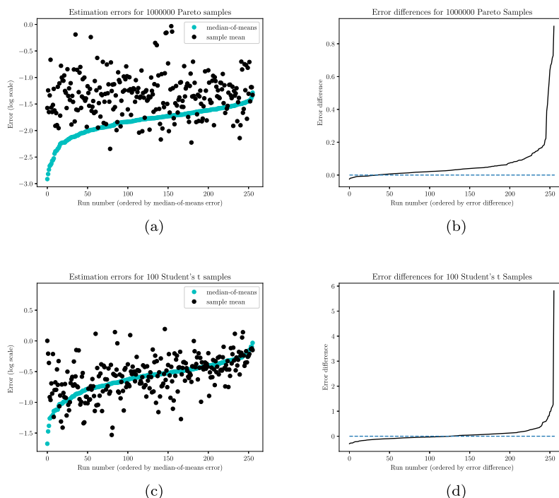
Fig 2: Comparison of errors corresponding to the median-of-means and sample mean estimator over 256 runs of the experiment. In (a) the sample of size N = 10^6 consists of i.i.d. random vectors in \mathbb{R}^2 with independent Pareto-distributed entries possessing only 2.1 moments. Each run computes the median-of-means estimator using partition into k = 1000 groups, as well as the usual sample mean. In (b), the ordered differences between the error of the sample mean and the median-of-means over all 256 runs illustrates robustness. Positive error differences in (b) indicate lower error for the median-of-means, and negative error differences occur when the sample mean provided a better estimate. Images (c) and (d) illustrate a similar experiment that was performed for two-dimensional random vectors with independent entries with Student's t -distribution with 2 degrees of freedom. In this case, the sample size is N = 100 and the number of groups is k = 10 .
