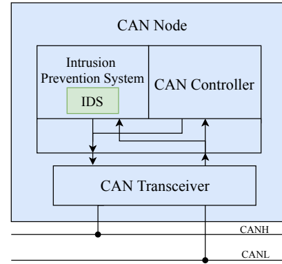
Figure 4: ECU Architecture
