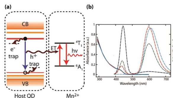
Fig. 1 (a) Energy transfer (ET) pathway in Mn-doped QDs. Energy transfer competes with exciton recombination and electron/hole trapping. (b) Absorption (solid line) and photoluminescence (dashed line) spectra of Mn-doped CdS/ZnS core/shell QDs with varying doping concentrations. Reproduced with permission from ref. 98. Copyright American Chemical Society (2010).
