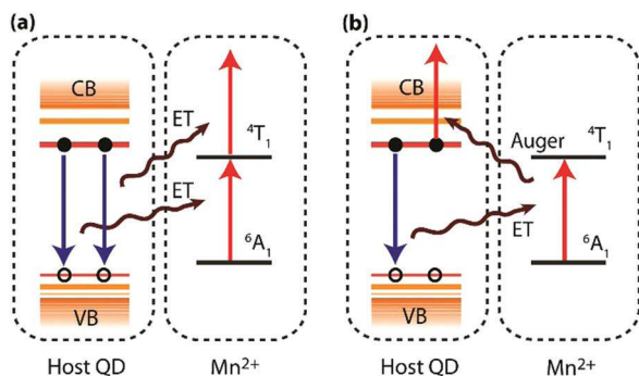
Fig. 5 Photophysical pathways that generate hot electrons in Mn-doped QDs. (a) Hot electrons are generated by consecutive exciton-to-Mn energy transfer. (b) Hot electrons are generated by exciton-to-Mn energy transfer followed by Auger type back energy transfer from \text{Mn}^{2+} to conduction band electrons.
