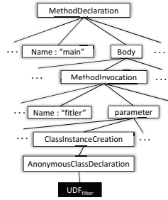
(b) Generated AST
