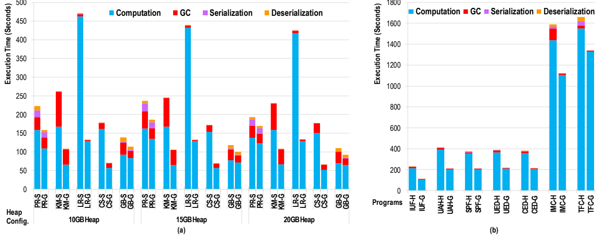
Figure 6. Runtime comparisons for Spark (a) and Hadoop (b); each group compares running time, for each program, between the baseline on the left and the Gerenuk version on the right; each bar is further broken down into four components: computation (in blue), GC (in red), serialization (in purple), and deserialization (in orange).
