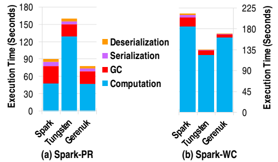
Figure 8. Comparison with Tungsten.
